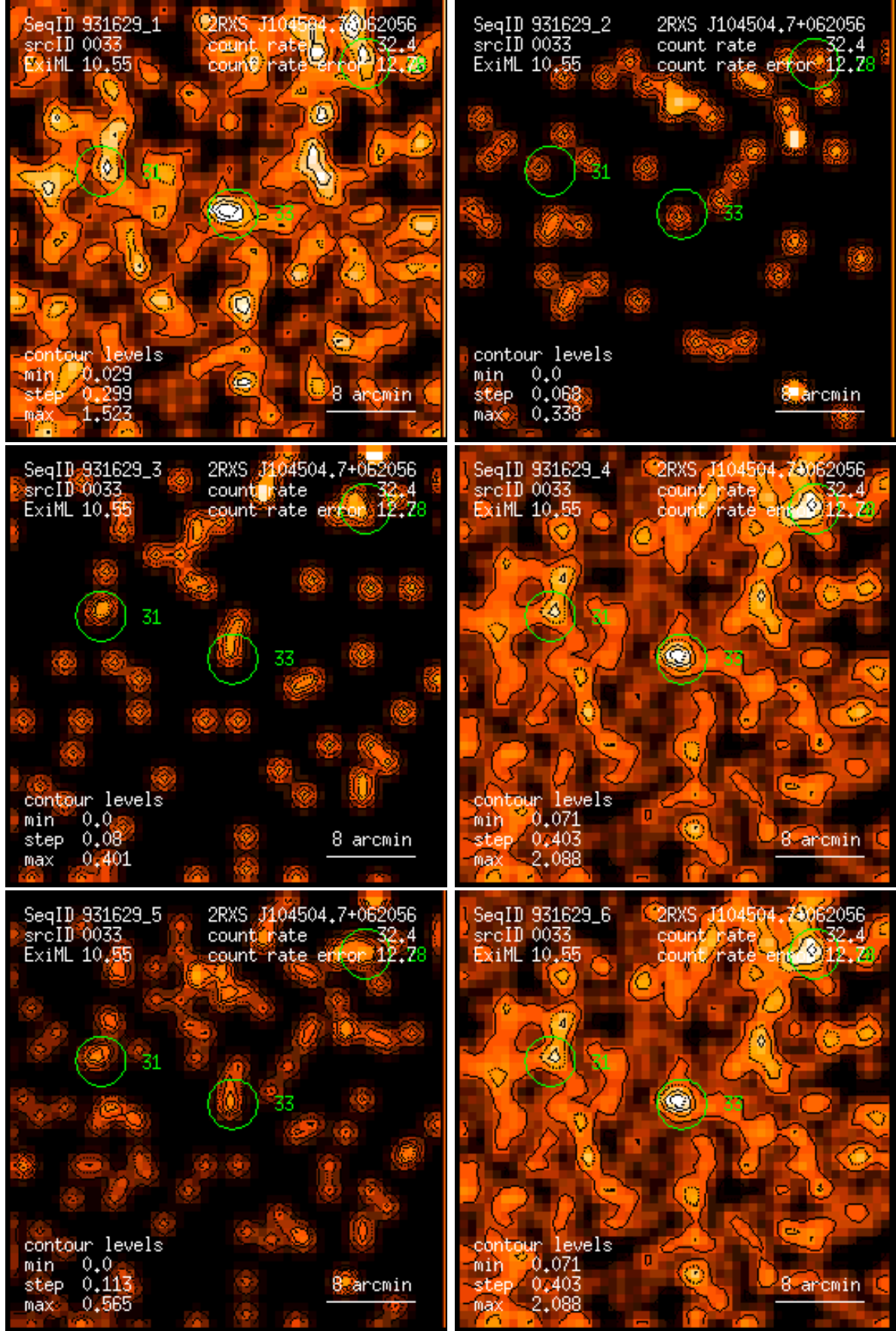
Figure 33: RASS 931629: detection 0033: band rate images, Gaussian filter: (1) PSPC channels 11 – 41, (2) 52 – 90, (3) 91 – 201, (4) 11 – 235, (5) 52 – 201, (6) 11 – 201. Broad band rates in counts/ks. Band rate contour levels in counts/ks/arcmin 2 .
