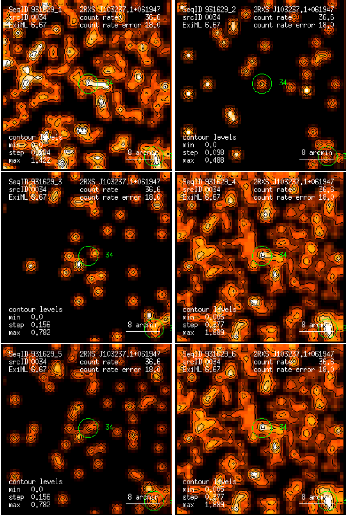
Figure 34: RASS 931629: detection 0034: band rate images, Gaussian filter: (1) PSPC channels 11 – 41, (2) 52 – 90, (3) 91 – 201, (4) 11 – 235, (5) 52 – 201, (6) 11 – 201. Broad band rates in counts/ks. Band rate contour levels in counts/ks/arcmin 2 .
