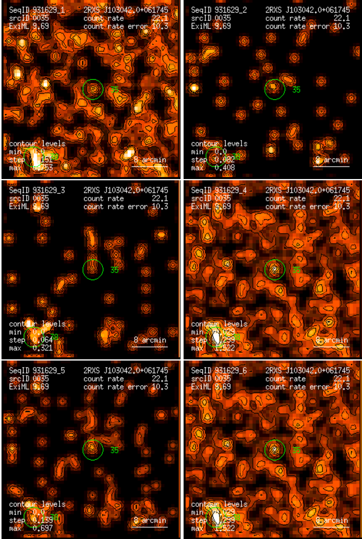
Figure 35: RASS 931629: detection 0035: band rate images, Gaussian filter: (1) PSPC channels 11 – 41, (2) 52 – 90, (3) 91 – 201, (4) 11 – 235, (5) 52 – 201, (6) 11 – 201. Broad band rates in counts/ks. Band rate contour levels in counts/ks/arcmin 2 .
