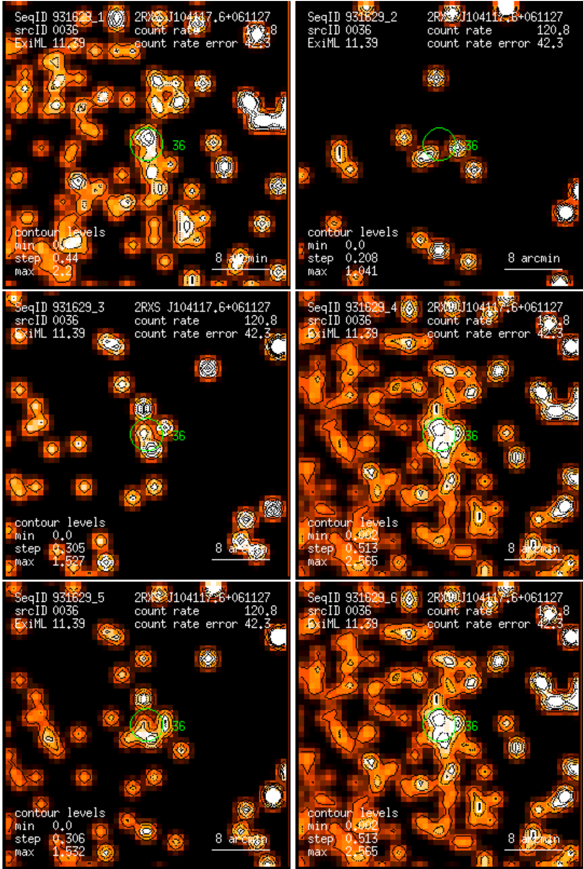
Figure 36: RASS 931629: detection 0036: band rate images, Gaussian filter: (1) PSPC channels 11 – 41, (2) 52 – 90, (3) 91 – 201, (4) 11 – 235, (5) 52 – 201, (6) 11 – 201. Broad band rates in counts/ks. Band rate contour levels in counts/ks/arcmin 2 .
