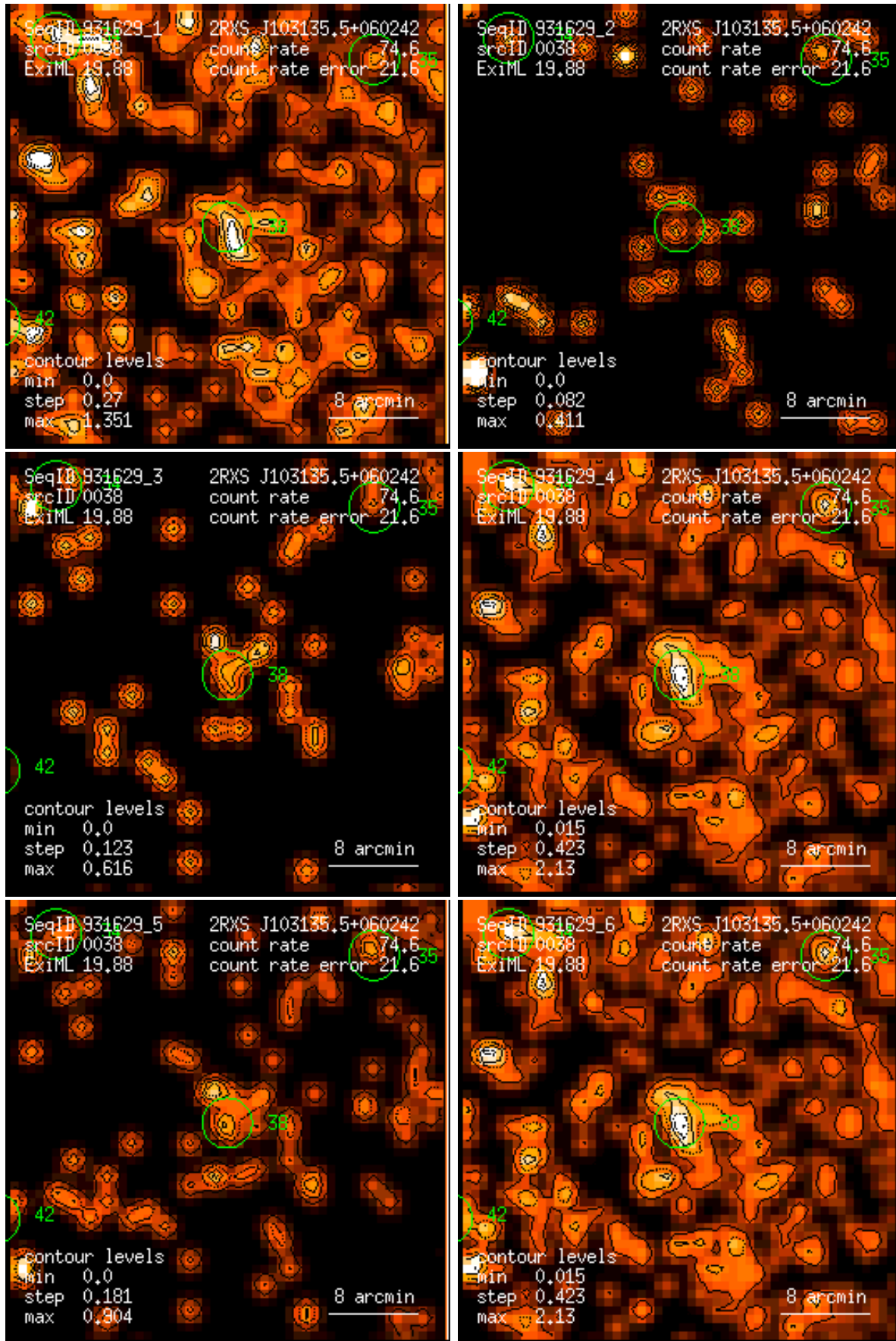
Figure 38: RASS 931629: detection 0038: band rate images, Gaussian filter: (1) PSPC channels 11 – 41, (2) 52 – 90, (3) 91 – 201, (4) 11 – 235, (5) 52 – 201, (6) 11 – 201. Broad band rates in counts/ks. Band rate contour levels in counts/ks/arcmin 2 .
