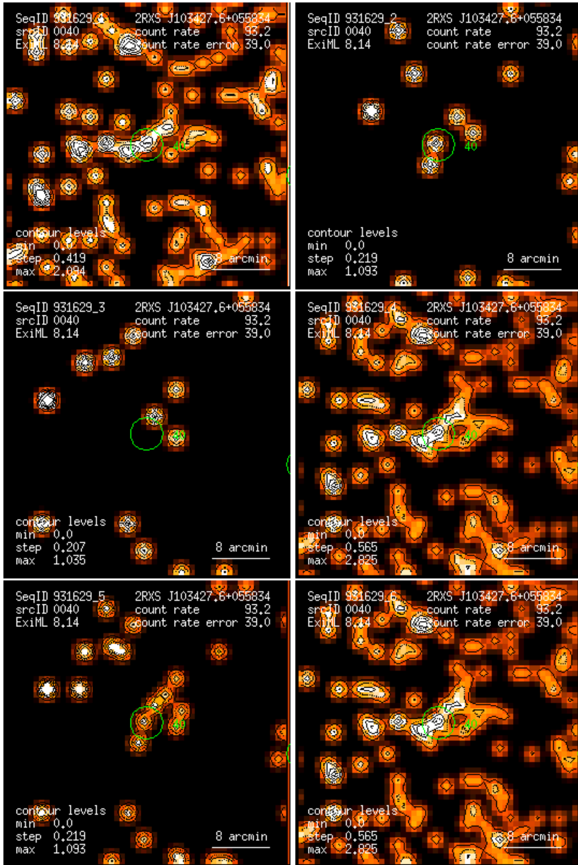
Figure 40: RASS 931629: detection 0040: band rate images, Gaussian filter: (1) PSPC channels 11 – 41, (2) 52 – 90, (3) 91 – 201, (4) 11 – 235, (5) 52 – 201, (6) 11 – 201. Broad band rates in counts/ks. Band rate contour levels in counts/ks/arcmin 2 .
