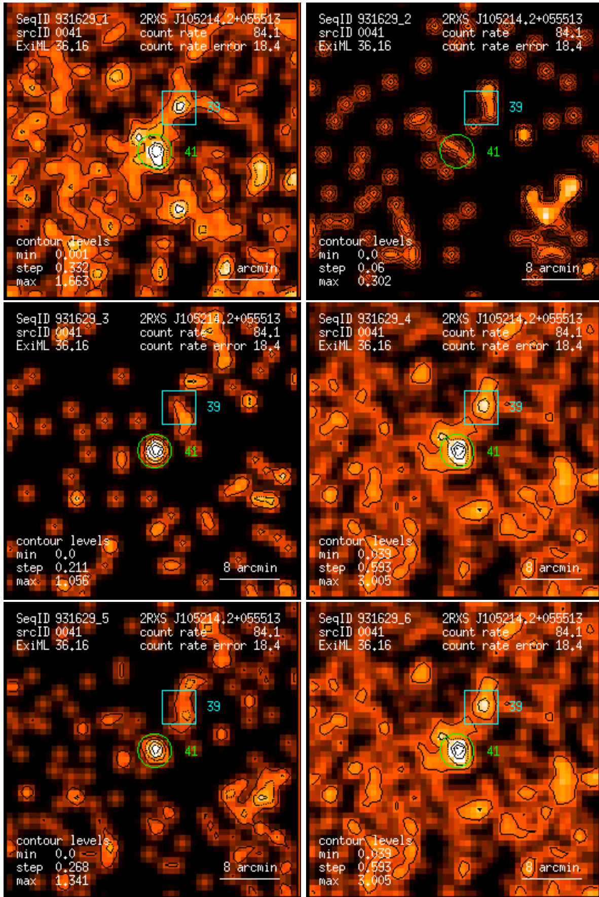
Figure 41: RASS 931629: detection 0041: band rate images, Gaussian filter: (1) PSPC channels 11 – 41, (2) 52 – 90, (3) 91 – 201, (4) 11 – 235, (5) 52 – 201, (6) 11 – 201. Broad band rates in counts/ks. Band rate contour levels in counts/ks/arcmin 2 .
