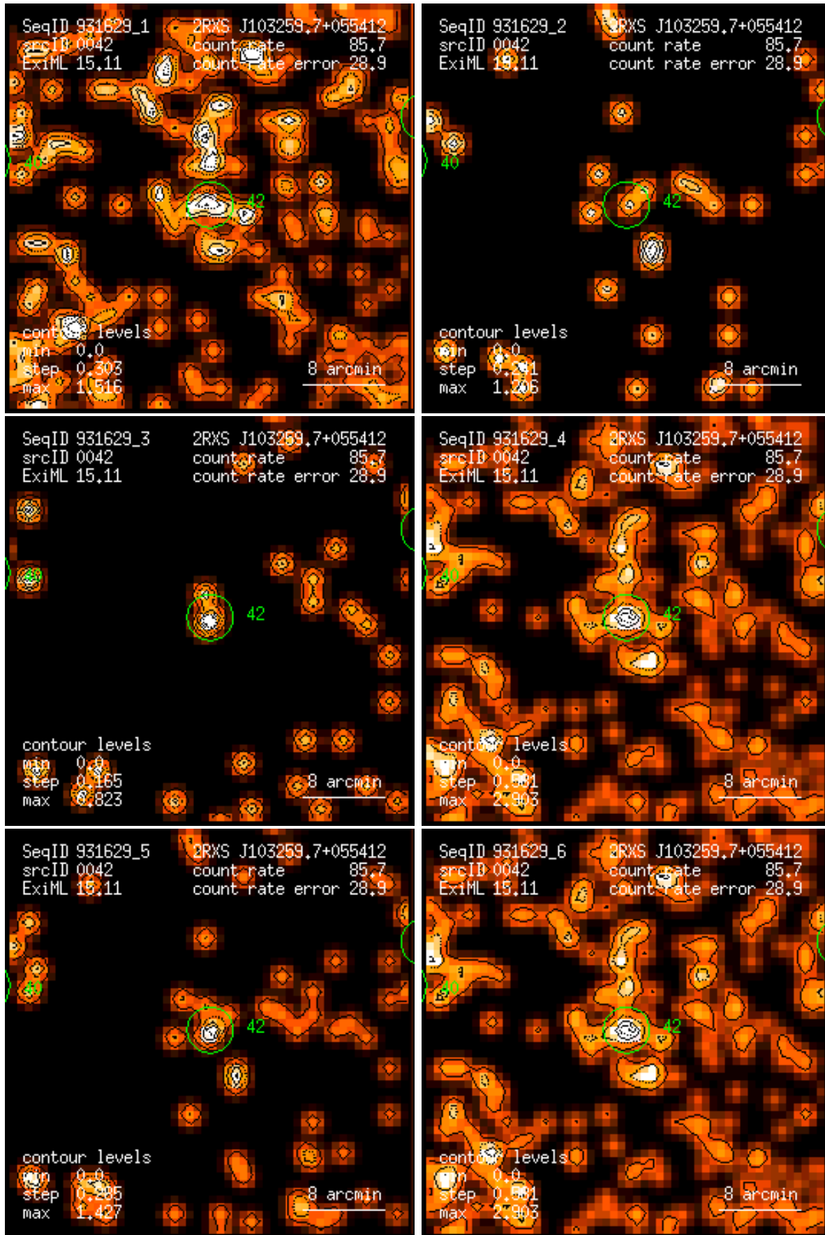
Figure 42: RASS 931629: detection 0042: band rate images, Gaussian filter: (1) PSPC channels 11 – 41, (2) 52 – 90, (3) 91 – 201, (4) 11 – 235, (5) 52 – 201, (6) 11 – 201. Broad band rates in counts/ks. Band rate contour levels in counts/ks/arcmin 2 .
