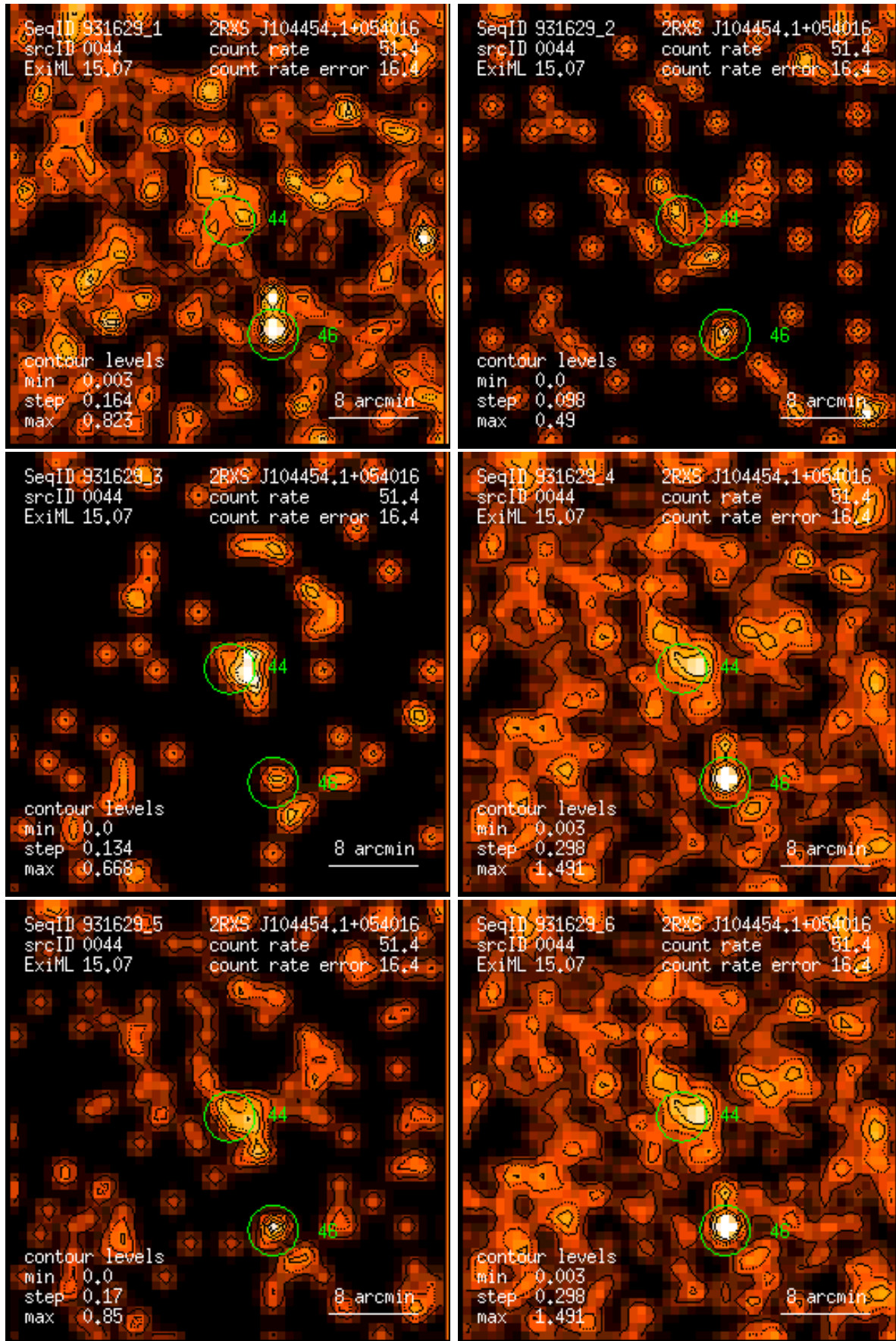
Figure 44: RASS 931629: detection 0044: band rate images, Gaussian filter: (1) PSPC channels 11 – 41, (2) 52 – 90, (3) 91 – 201, (4) 11 – 235, (5) 52 – 201, (6) 11 – 201. Broad band rates in counts/ks. Band rate contour levels in counts/ks/arcmin 2 .
