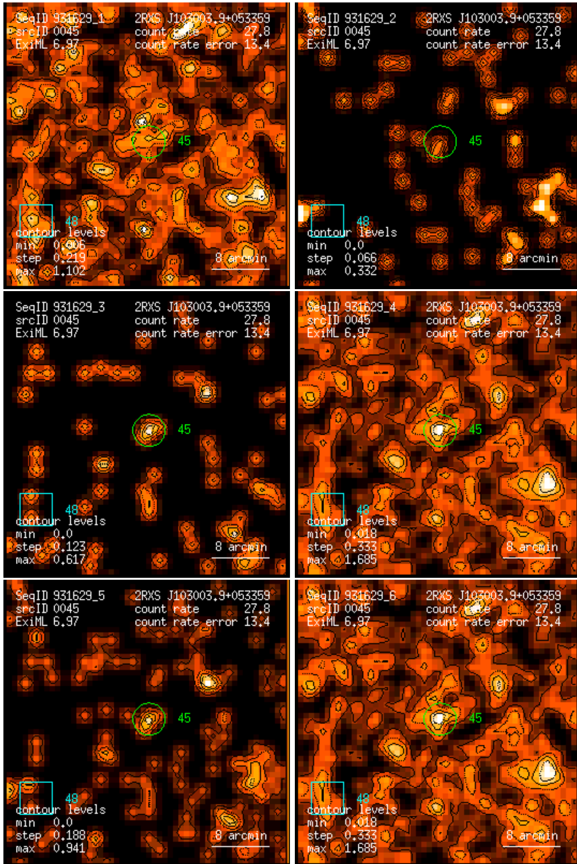
Figure 45: RASS 931629: detection 0045: band rate images, Gaussian filter: (1) PSPC channels 11 – 41, (2) 52 – 90, (3) 91 – 201, (4) 11 – 235, (5) 52 – 201, (6) 11 – 201. Broad band rates in counts/ks. Band rate contour levels in counts/ks/arcmin 2 .
