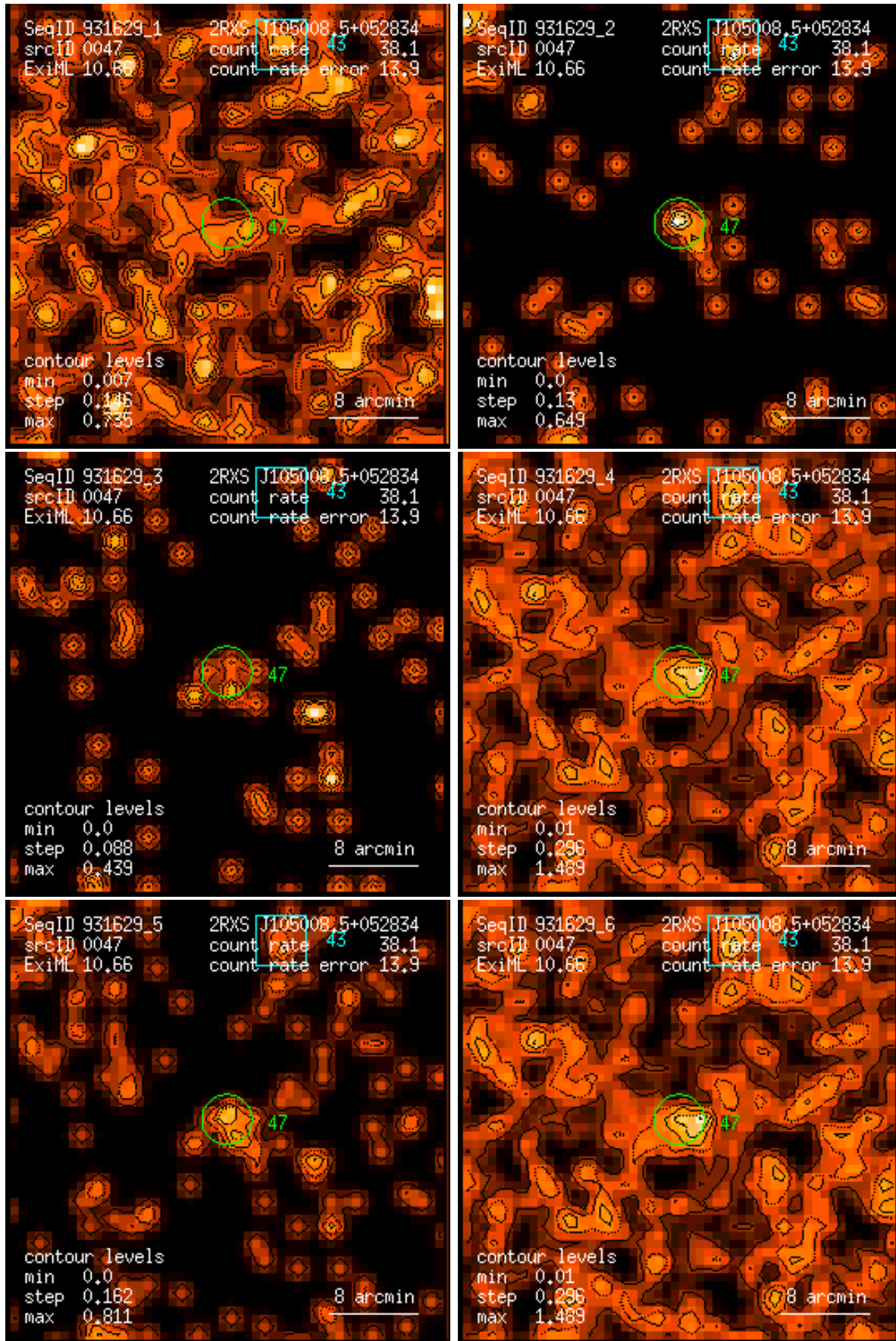
Figure 47: RASS 931629: detection 0047: band rate images, Gaussian filter: (1) PSPC channels 11 – 41, (2) 52 – 90, (3) 91 – 201, (4) 11 – 235, (5) 52 – 201, (6) 11 – 201. Broad band rates in counts/ks. Band rate contour levels in counts/ks/arcmin 2 .
