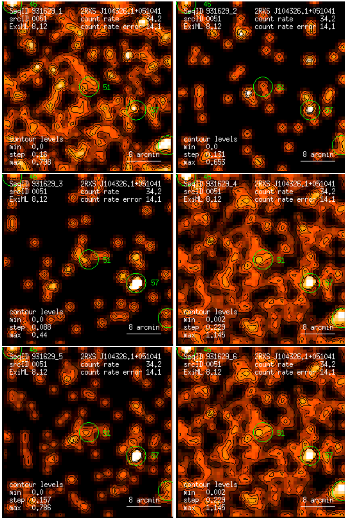
Figure 51: RASS 931629: detection 0051: band rate images, Gaussian filter: (1) PSPC channels 11 – 41, (2) 52 – 90, (3) 91 – 201, (4) 11 – 235, (5) 52 – 201, (6) 11 – 201. Broad band rates in counts/ks. Band rate contour levels in counts/ks/arcmin 2 .
