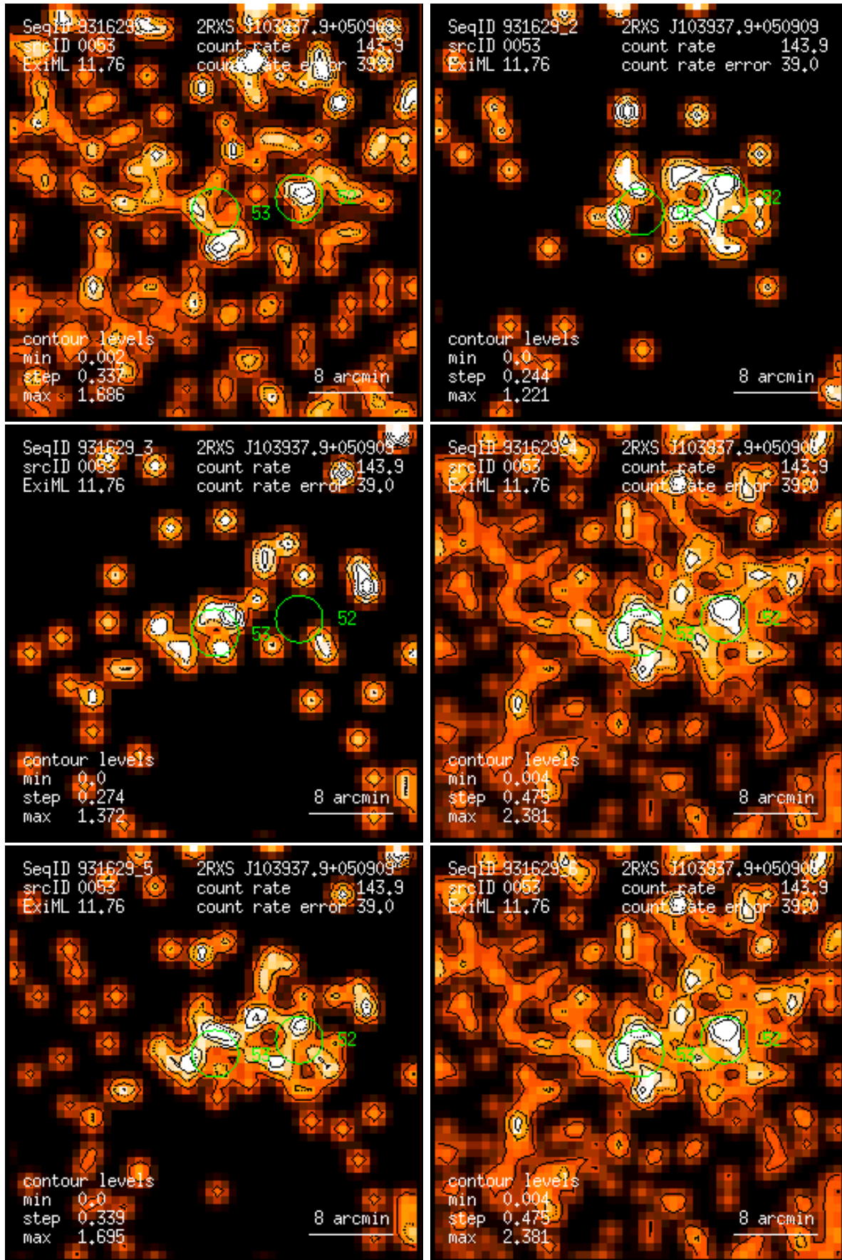
Figure 53: RASS 931629: detection 0053: band rate images, Gaussian filter: (1) PSPC channels 11 – 41, (2) 52 – 90, (3) 91 – 201, (4) 11 – 235, (5) 52 – 201, (6) 11 – 201. Broad band rates in counts/ks. Band rate contour levels in counts/ks/arcmin 2 .
