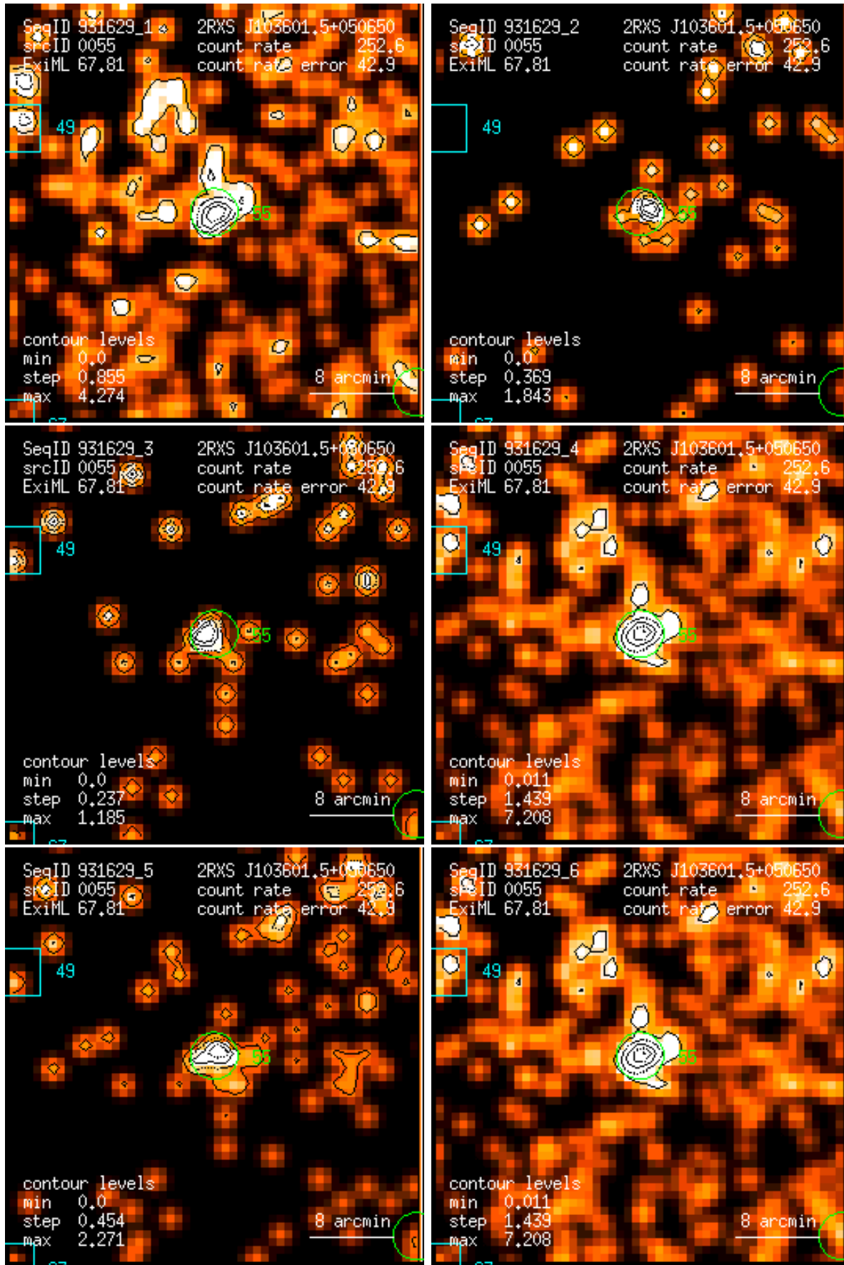
Figure 55: RASS 931629: detection 0055: band rate images, Gaussian filter: (1) PSPC channels 11 – 41, (2) 52 – 90, (3) 91 – 201, (4) 11 – 235, (5) 52 – 201, (6) 11 – 201. Broad band rates in counts/ks. Band rate contour levels in counts/ks/arcmin 2 .
