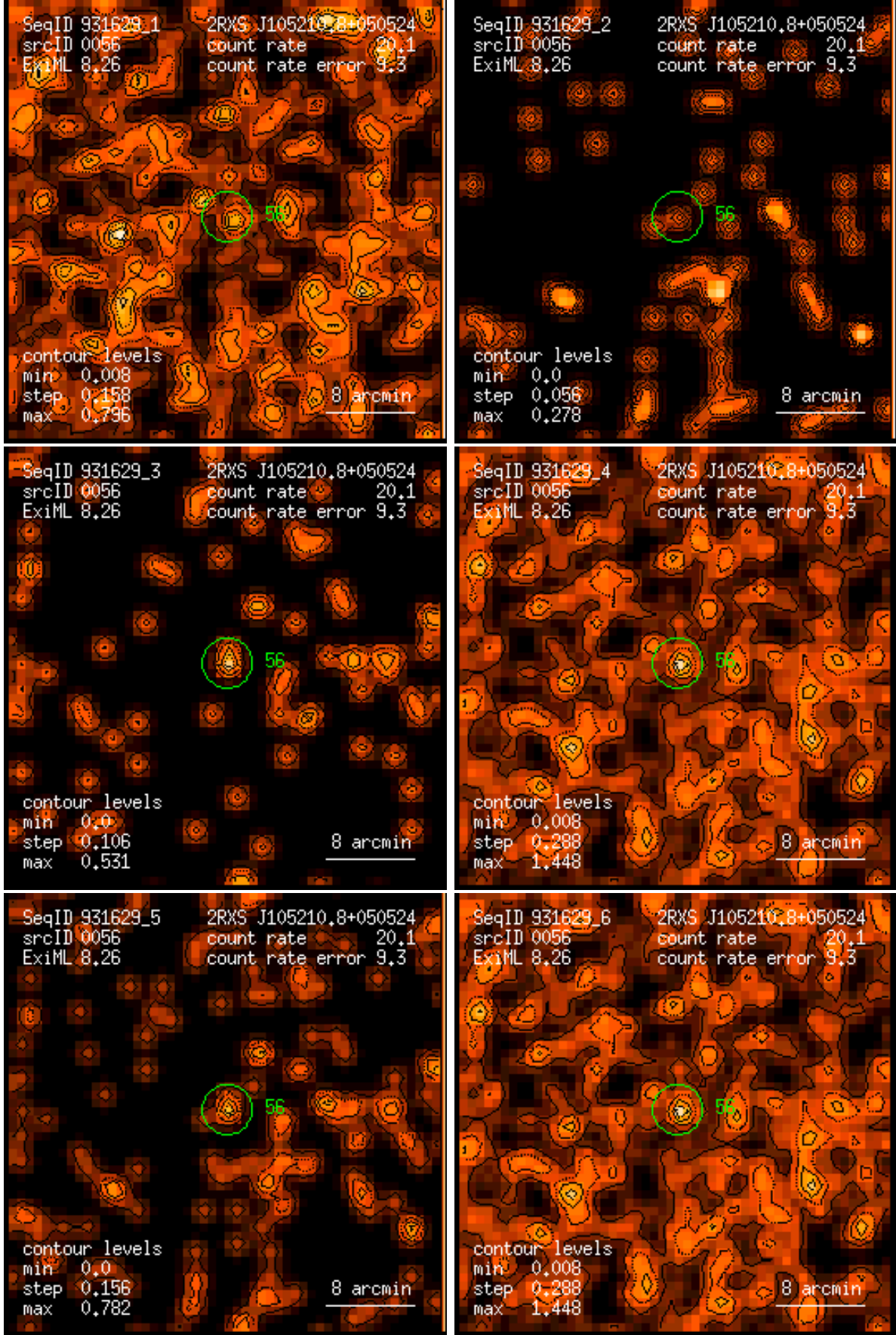
Figure 56: RASS 931629: detection 0056: band rate images, Gaussian filter: (1) PSPC channels 11 – 41, (2) 52 – 90, (3) 91 – 201, (4) 11 – 235, (5) 52 – 201, (6) 11 – 201. Broad band rates in counts/ks. Band rate contour levels in counts/ks/arcmin 2 .
