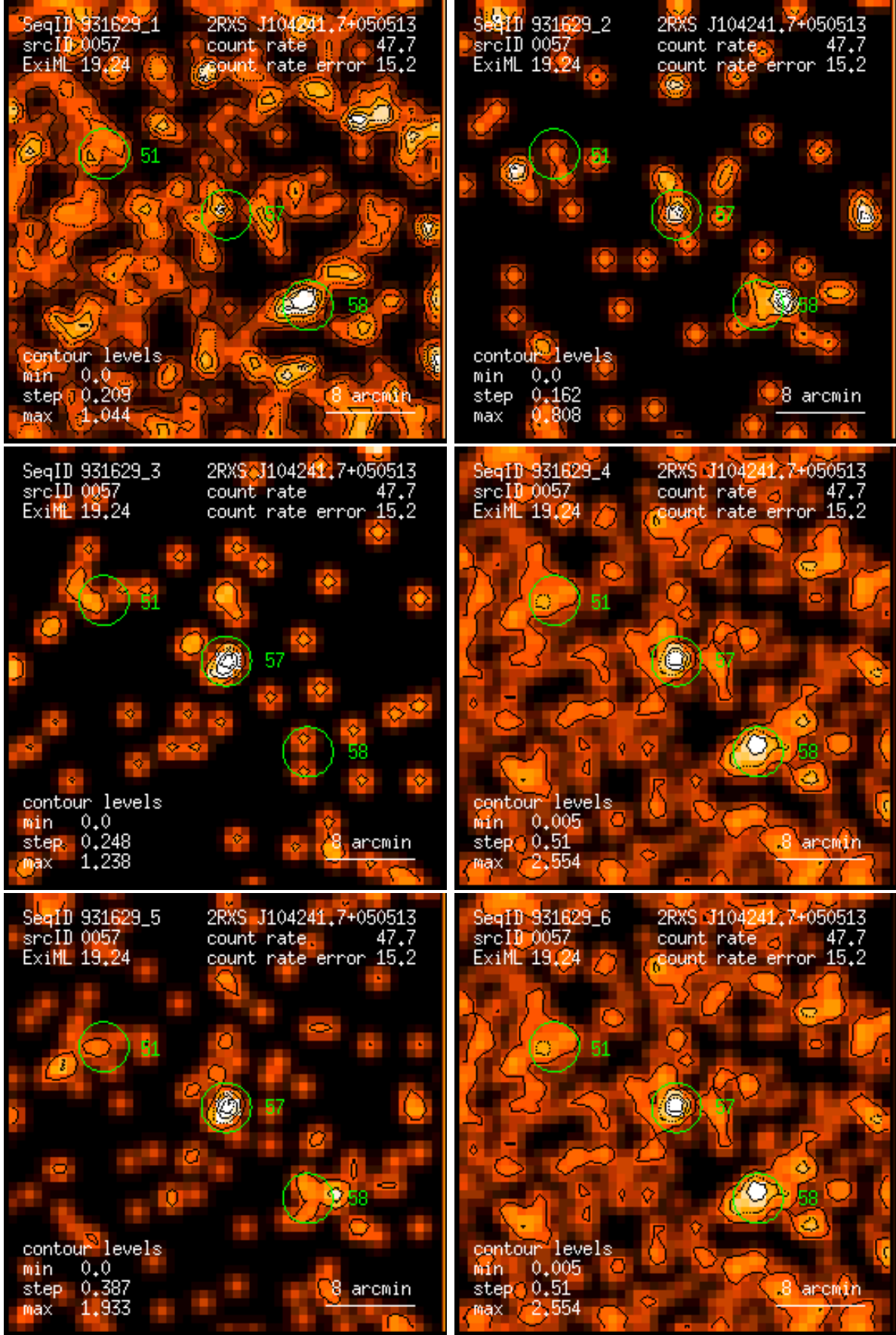
Figure 57: RASS 931629: detection 0057: band rate images, Gaussian filter: (1) PSPC channels 11 – 41, (2) 52 – 90, (3) 91 – 201, (4) 11 – 235, (5) 52 – 201, (6) 11 – 201. Broad band rates in counts/ks. Band rate contour levels in counts/ks/arcmin 2 .
