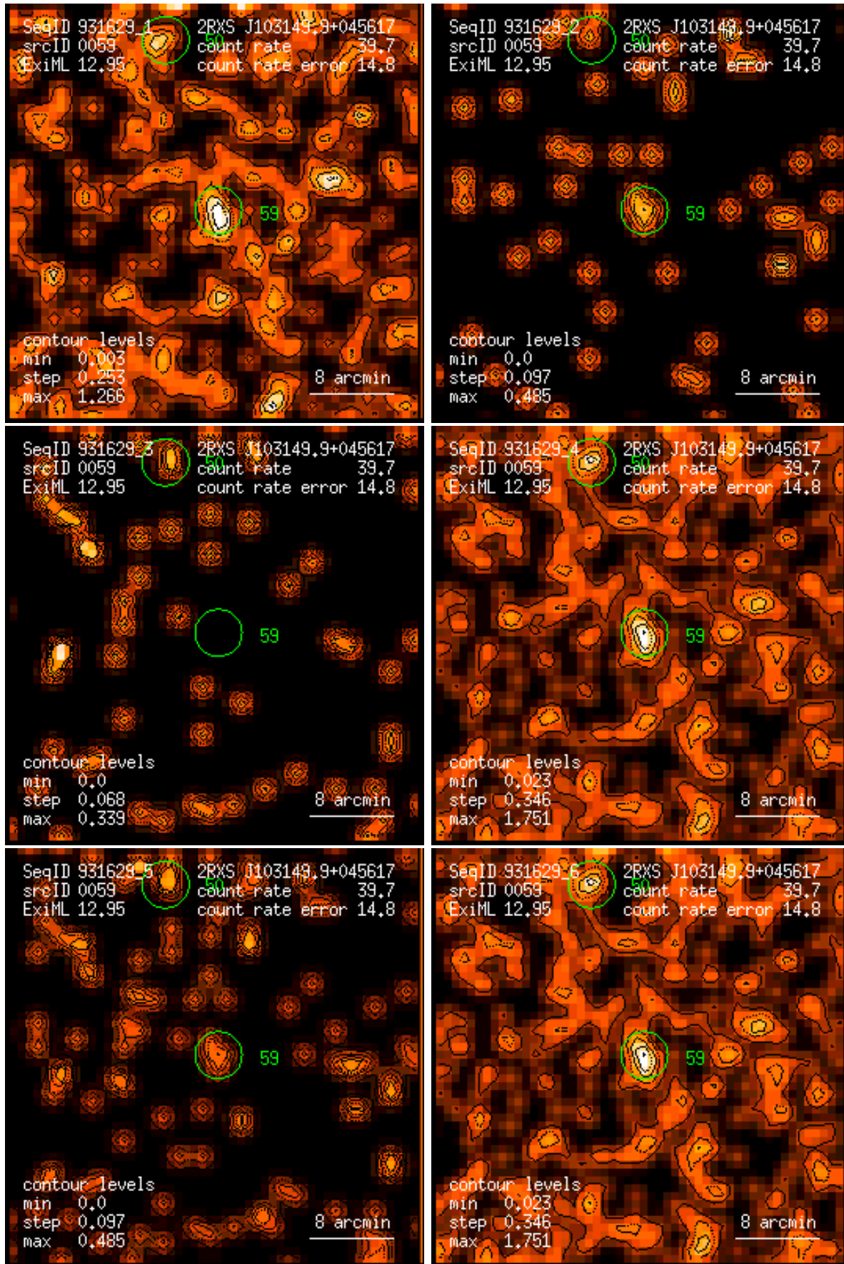
Figure 59: RASS 931629: detection 0059: band rate images, Gaussian filter: (1) PSPC channels 11 – 41, (2) 52 – 90, (3) 91 – 201, (4) 11 – 235, (5) 52 – 201, (6) 11 – 201. Broad band rates in counts/ks. Band rate contour levels in counts/ks/arcmin 2 .
