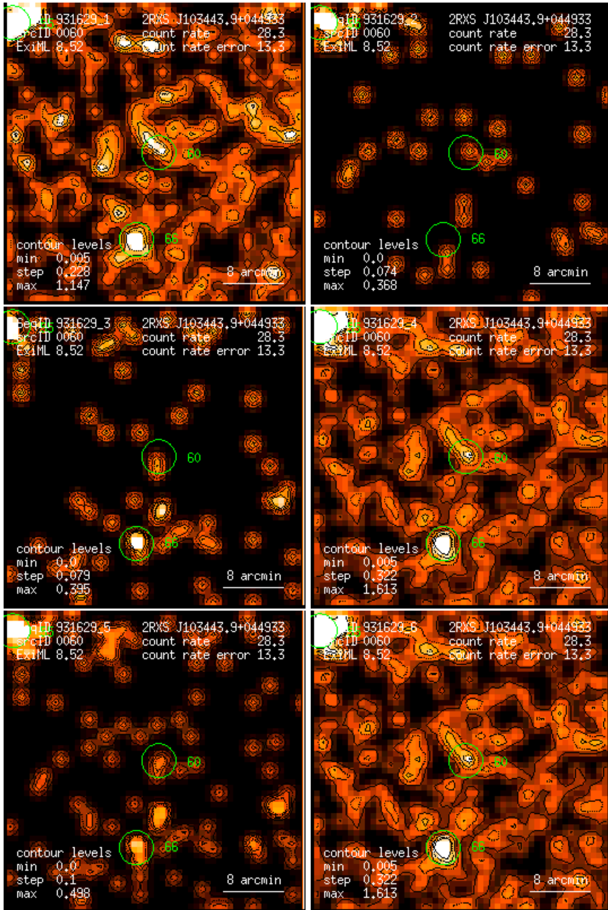
Figure 60: RASS 931629: detection 0060: band rate images, Gaussian filter: (1) PSPC channels 11 – 41, (2) 52 – 90, (3) 91 – 201, (4) 11 – 235, (5) 52 – 201, (6) 11 – 201. Broad band rates in counts/ks. Band rate contour levels in counts/ks/arcmin 2 .
