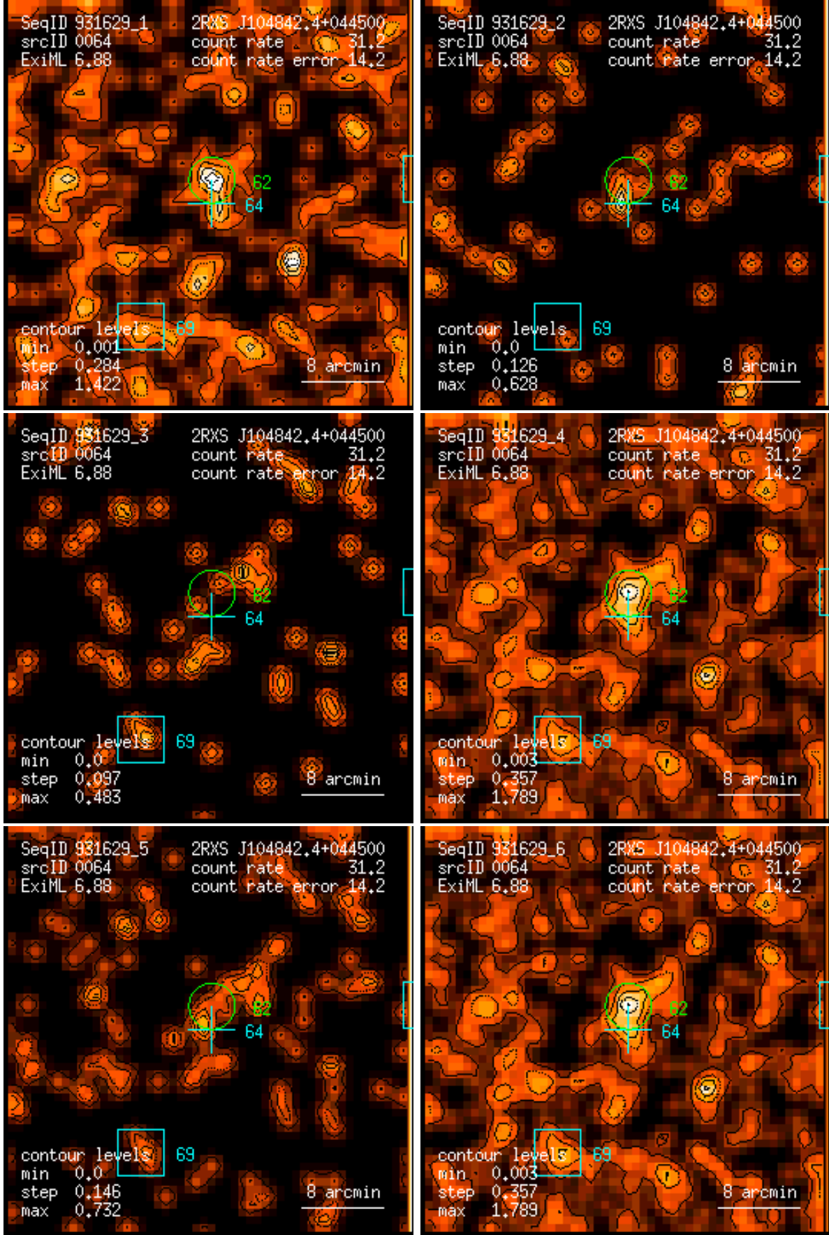
Figure 64: RASS 931629: detection 0064: band rate images, Gaussian filter: (1) PSPC channels 11 – 41, (2) 52 – 90, (3) 91 – 201, (4) 11 – 235, (5) 52 – 201, (6) 11 – 201. Broad band rates in counts/ks. Band rate contour levels in counts/ks/arcmin 2 .
