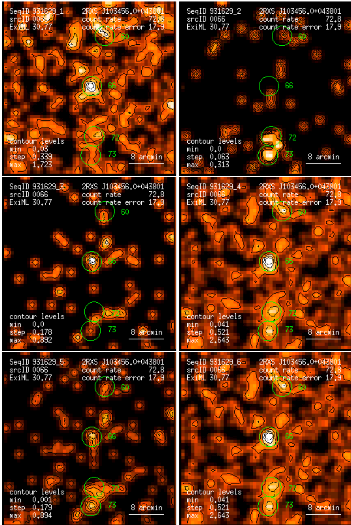
Figure 66: RASS 931629: detection 0066: band rate images, Gaussian filter: (1) PSPC channels 11 – 41, (2) 52 – 90, (3) 91 – 201, (4) 11 – 235, (5) 52 – 201, (6) 11 – 201. Broad band rates in counts/ks. Band rate contour levels in counts/ks/arcmin 2 .
