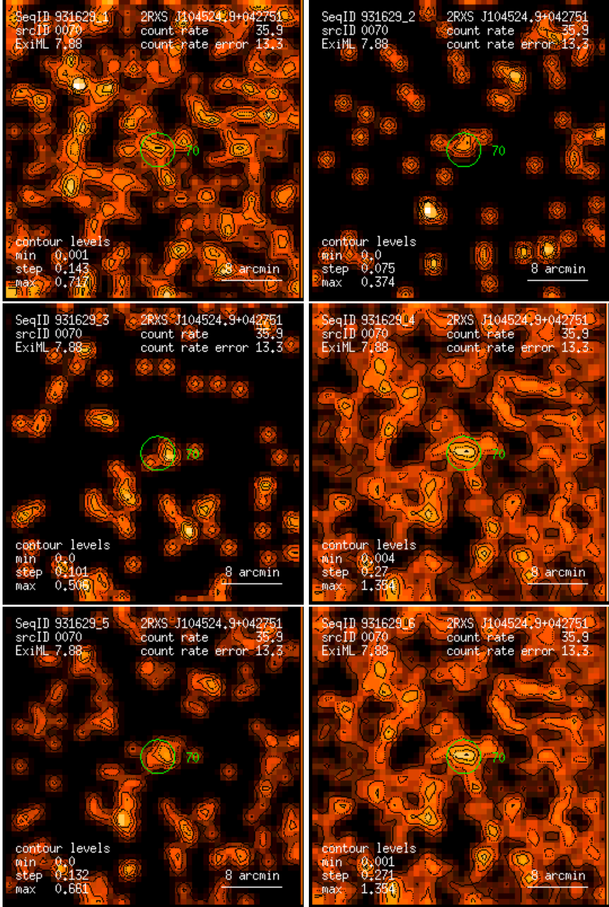
Figure 70: RASS 931629: detection 0070: band rate images, Gaussian filter: (1) PSPC channels 11 – 41, (2) 52 – 90, (3) 91 – 201, (4) 11 – 235, (5) 52 – 201, (6) 11 – 201. Broad band rates in counts/ks. Band rate contour levels in counts/ks/arcmin 2 .
