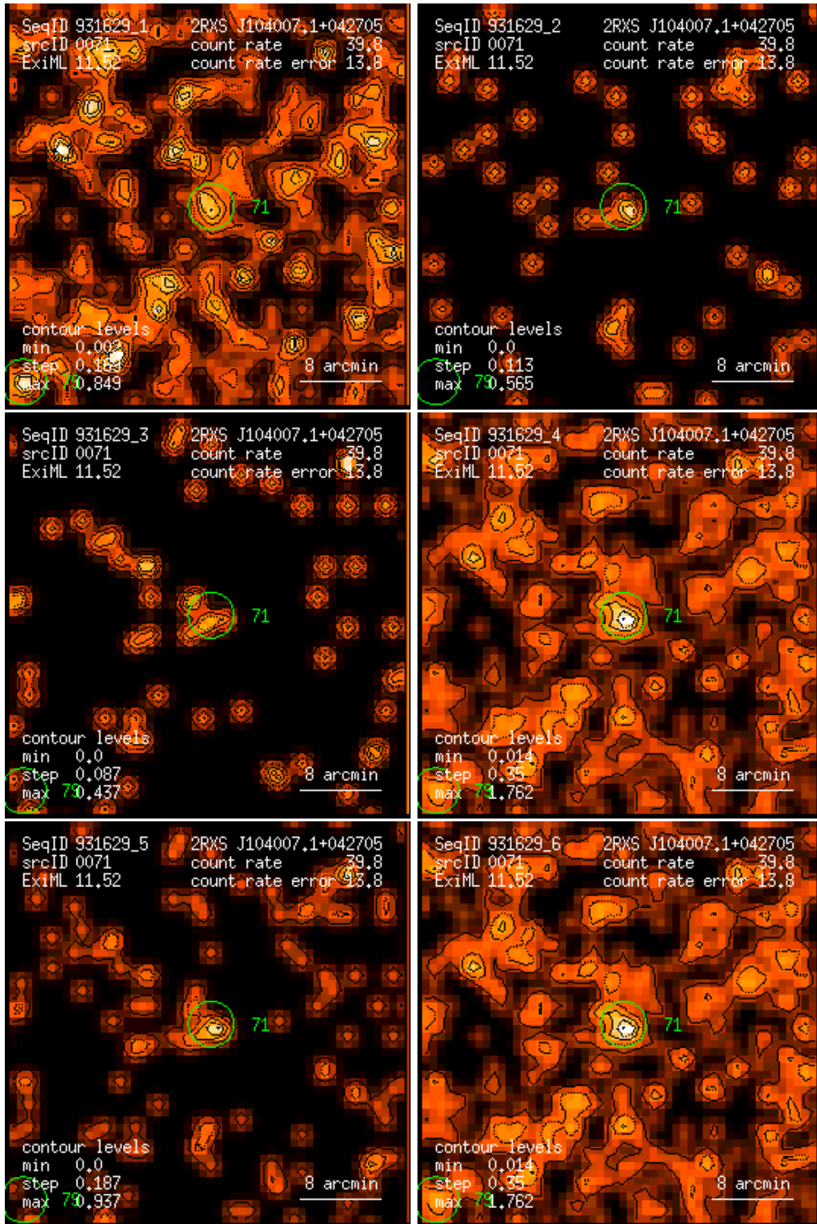
Figure 71: RASS 931629: detection 0071: band rate images, Gaussian filter: (1) PSPC channels 11 – 41, (2) 52 – 90, (3) 91 – 201, (4) 11 – 235, (5) 52 – 201, (6) 11 – 201. Broad band rates in counts/ks. Band rate contour levels in counts/ks/arcmin 2 .
