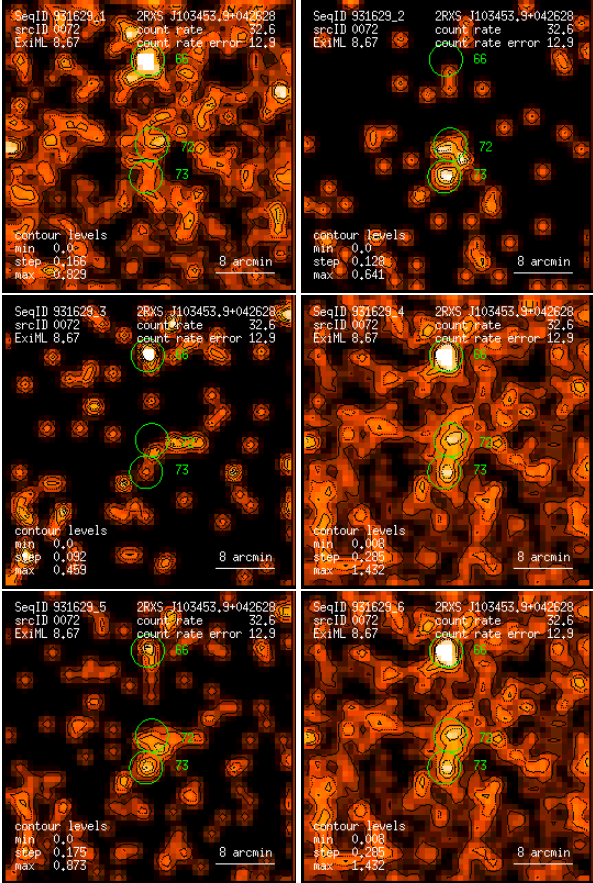
Figure 72: RASS 931629: detection 0072: band rate images, Gaussian filter: (1) PSPC channels 11 – 41, (2) 52 – 90, (3) 91 – 201, (4) 11 – 235, (5) 52 – 201, (6) 11 – 201. Broad band rates in counts/ks. Band rate contour levels in counts/ks/arcmin 2 .
