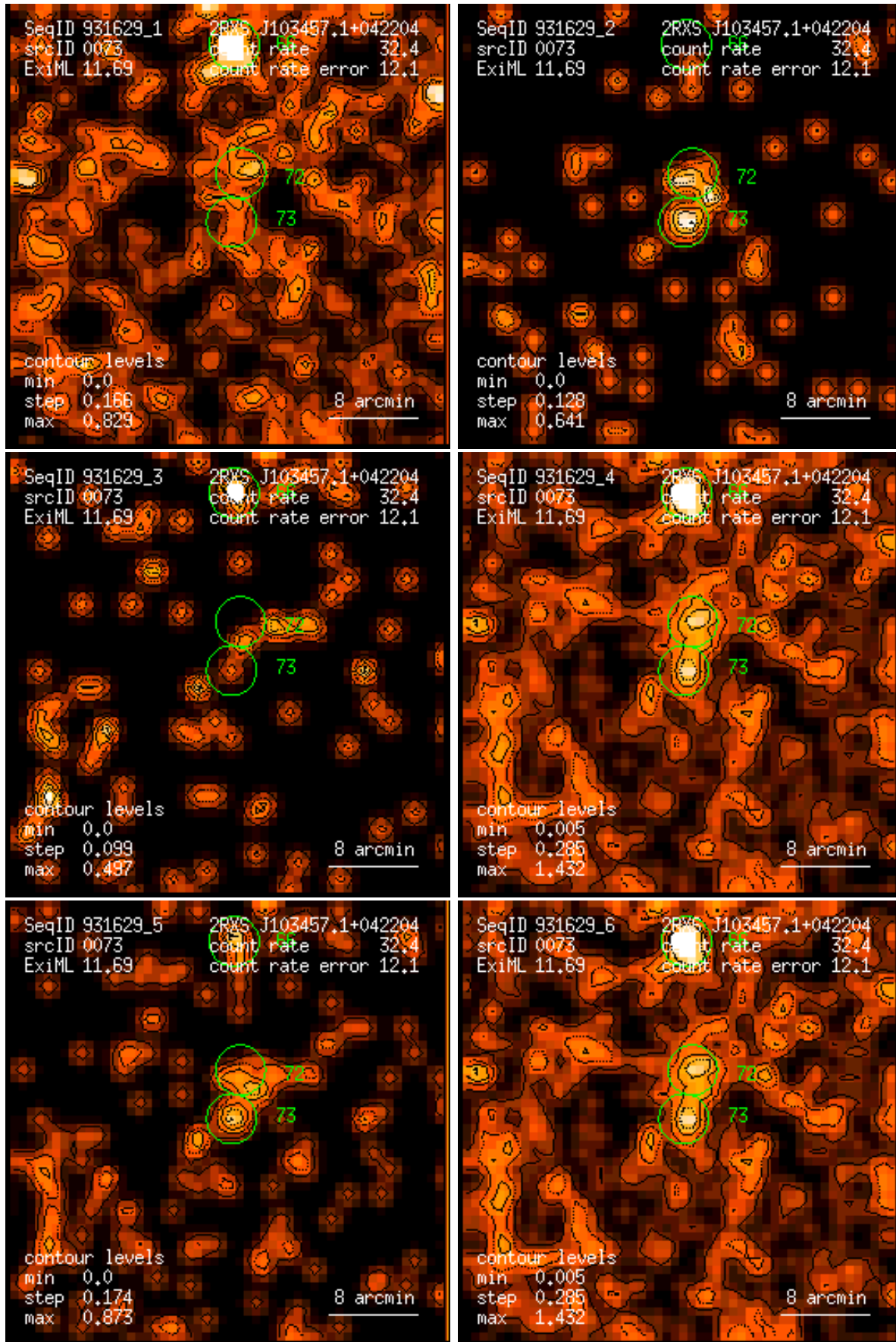
Figure 73: RASS 931629: detection 0073: band rate images, Gaussian filter: (1) PSPC channels 11 – 41, (2) 52 – 90, (3) 91 – 201, (4) 11 – 235, (5) 52 – 201, (6) 11 – 201. Broad band rates in counts/ks. Band rate contour levels in counts/ks/arcmin 2 .
