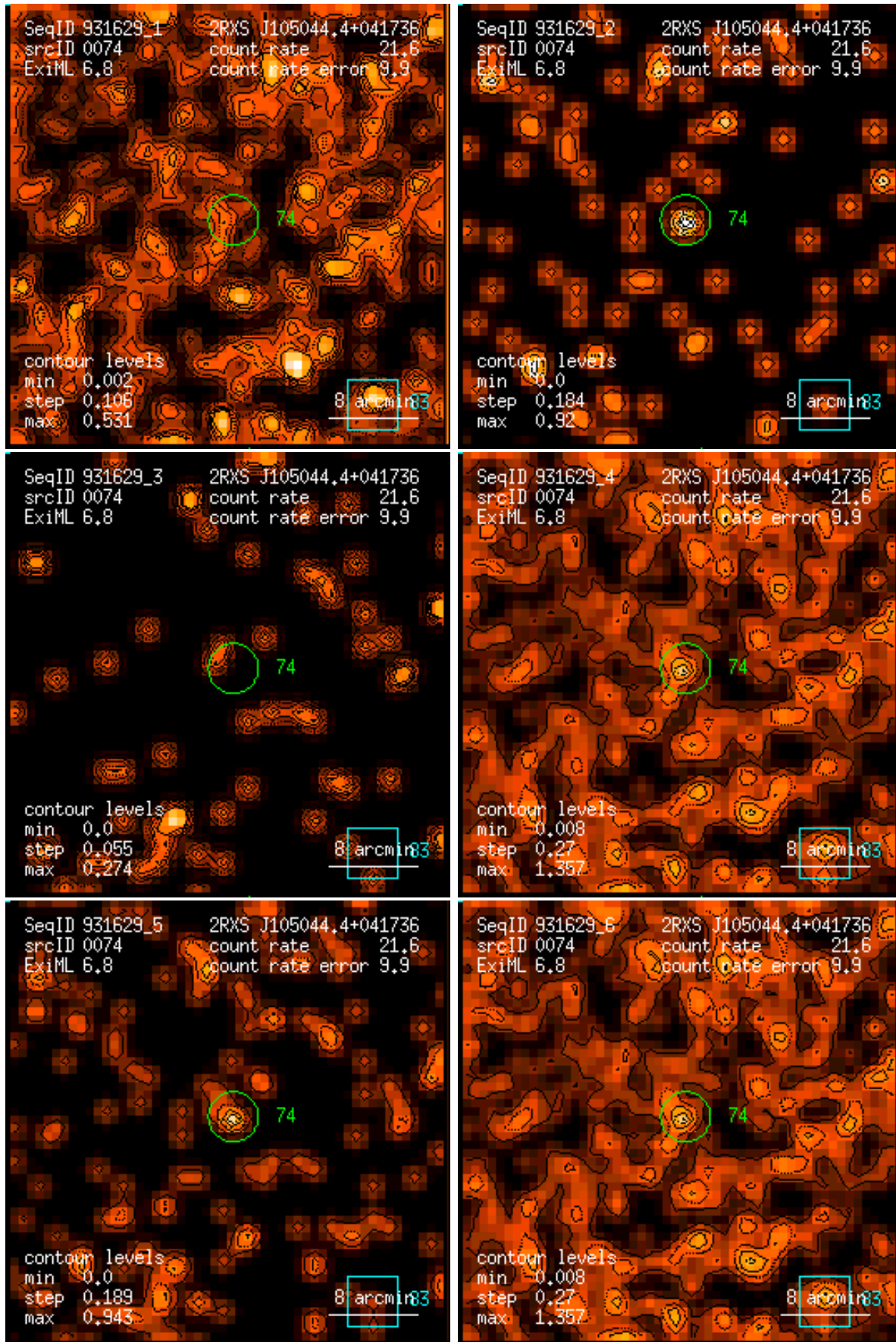
Figure 74: RASS 931629: detection 0074: band rate images, Gaussian filter: (1) PSPC channels 11 – 41, (2) 52 – 90, (3) 91 – 201, (4) 11 – 235, (5) 52 – 201, (6) 11 – 201. Broad band rates in counts/ks. Band rate contour levels in counts/ks/arcmin 2 .
