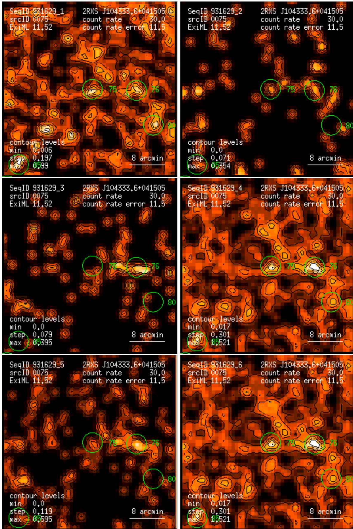
Figure 75: RASS 931629: detection 0075: band rate images, Gaussian filter: (1) PSPC channels 11 – 41, (2) 52 – 90, (3) 91 – 201, (4) 11 – 235, (5) 52 – 201, (6) 11 – 201. Broad band rates in counts/ks. Band rate contour levels in counts/ks/arcmin 2 .
