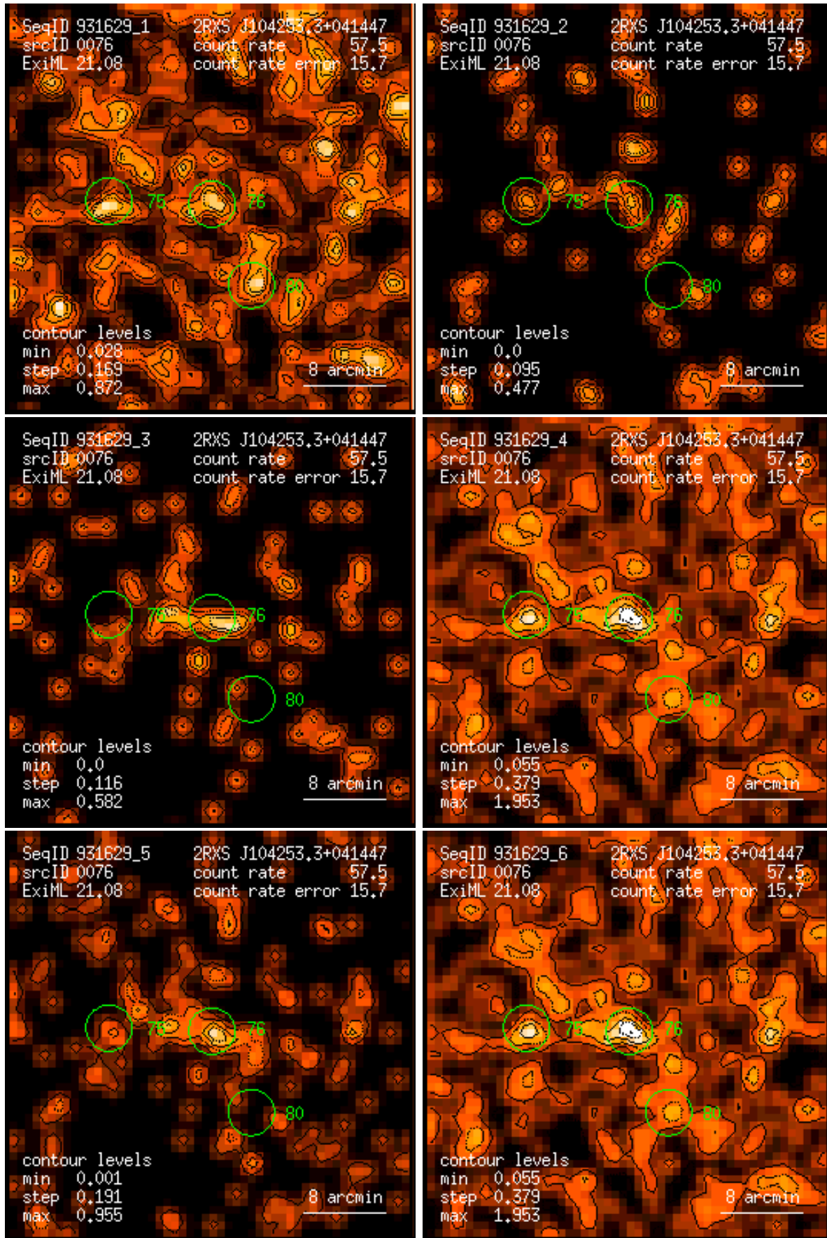
Figure 76: RASS 931629: detection 0076: band rate images, Gaussian filter: (1) PSPC channels 11 – 41, (2) 52 – 90, (3) 91 – 201, (4) 11 – 235, (5) 52 – 201, (6) 11 – 201. Broad band rates in counts/ks. Band rate contour levels in counts/ks/arcmin 2 .
