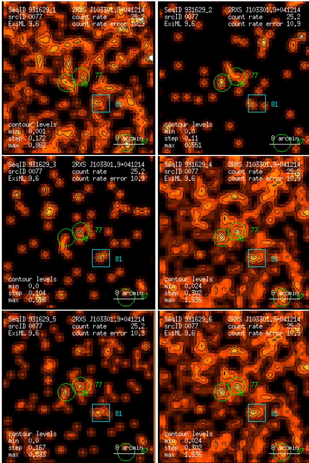
Figure 77: RASS 931629: detection 0077: band rate images, Gaussian filter: (1) PSPC channels 11 – 41, (2) 52 – 90, (3) 91 – 201, (4) 11 – 235, (5) 52 – 201, (6) 11 – 201. Broad band rates in counts/ks. Band rate contour levels in counts/ks/arcmin 2 .
