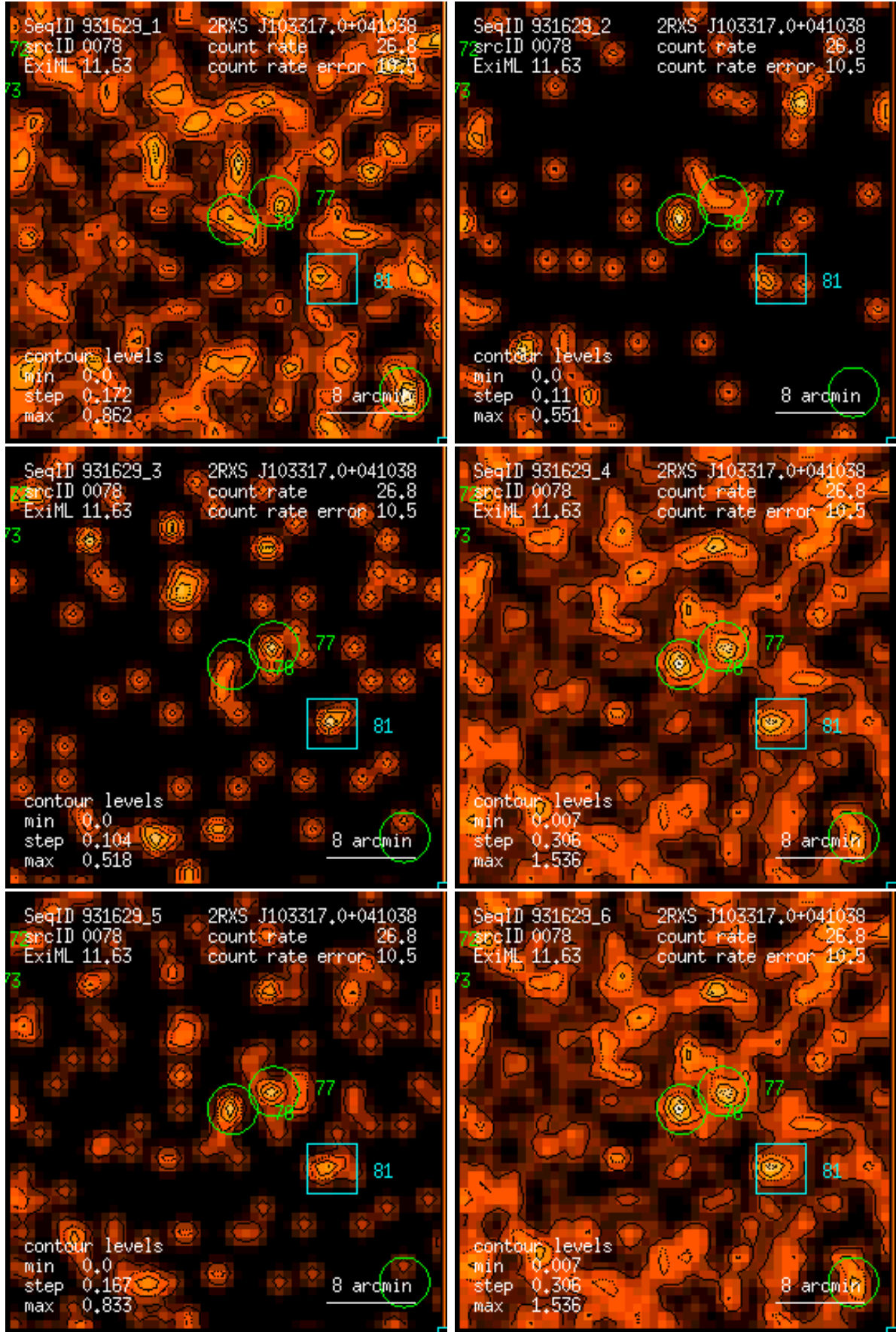
Figure 78: RASS 931629: detection 0078: band rate images, Gaussian filter: (1) PSPC channels 11 – 41, (2) 52 – 90, (3) 91 – 201, (4) 11 – 235, (5) 52 – 201, (6) 11 – 201. Broad band rates in counts/ks. Band rate contour levels in counts/ks/arcmin 2 .
