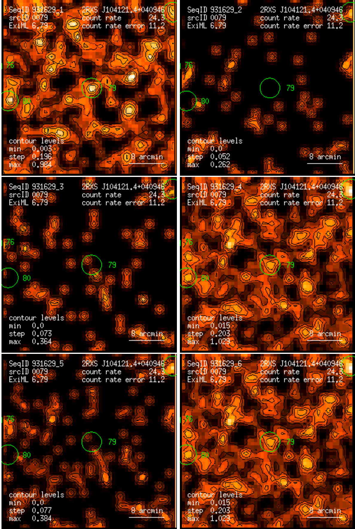
Figure 79: RASS 931629: detection 0079: band rate images, Gaussian filter: (1) PSPC channels 11 – 41, (2) 52 – 90, (3) 91 – 201, (4) 11 – 235, (5) 52 – 201, (6) 11 – 201. Broad band rates in counts/ks. Band rate contour levels in counts/ks/arcmin 2 .
