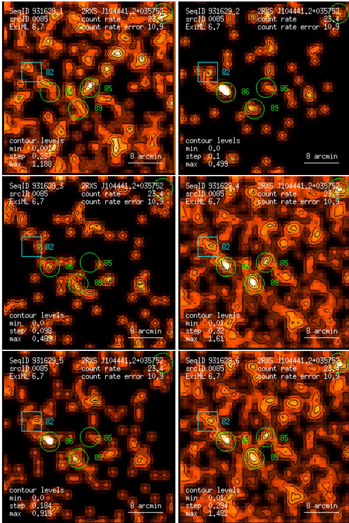
Figure 85: RASS 931629: detection 0085: band rate images, Gaussian filter: (1) PSPC channels 11 – 41, (2) 52 – 90, (3) 91 – 201, (4) 11 – 235, (5) 52 – 201, (6) 11 – 201. Broad band rates in counts/ks. Band rate contour levels in counts/ks/arcmin 2 .
