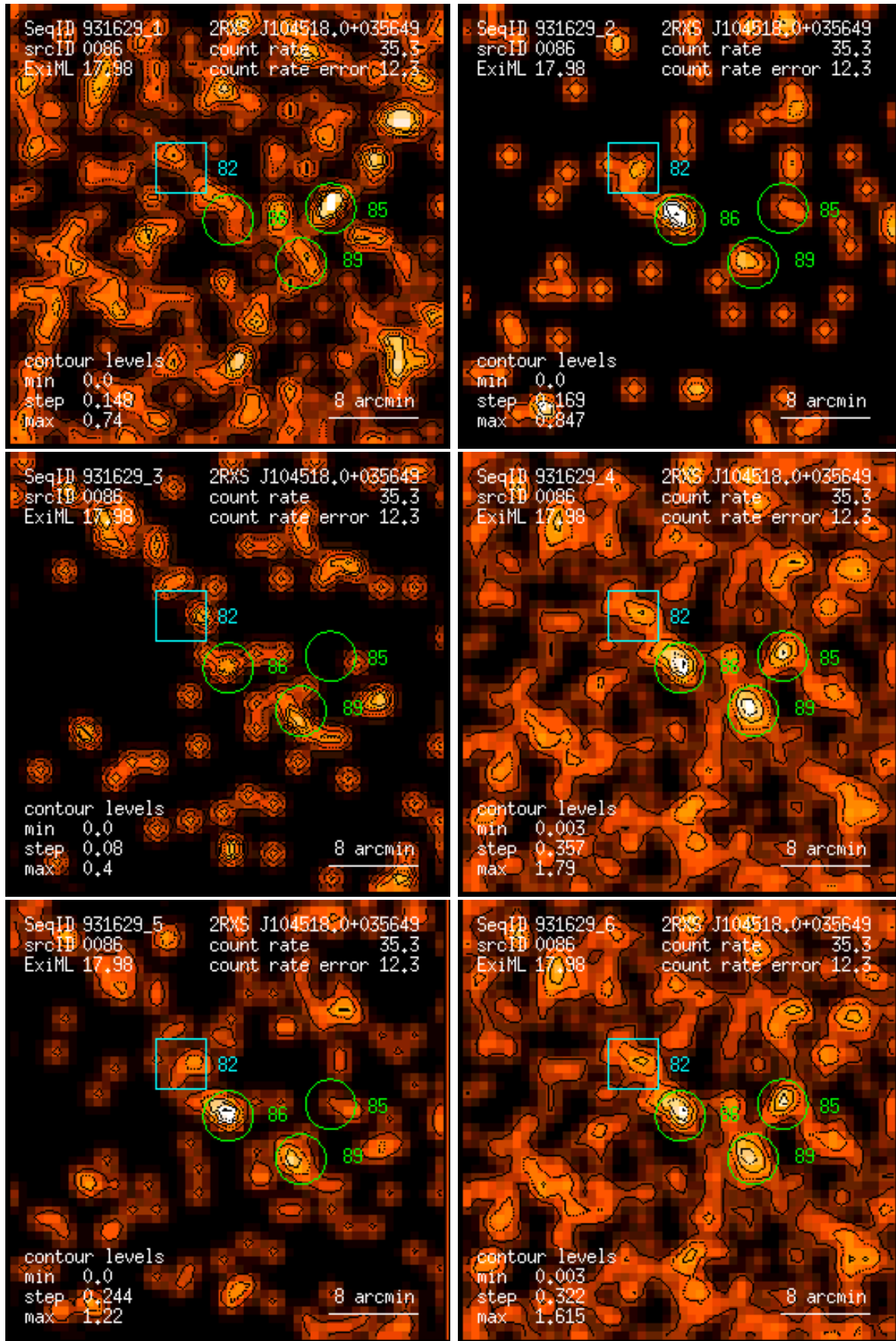
Figure 86: RASS 931629: detection 0086: band rate images, Gaussian filter: (1) PSPC channels 11 – 41, (2) 52 – 90, (3) 91 – 201, (4) 11 – 235, (5) 52 – 201, (6) 11 – 201. Broad band rates in counts/ks. Band rate contour levels in counts/ks/arcmin 2 .
