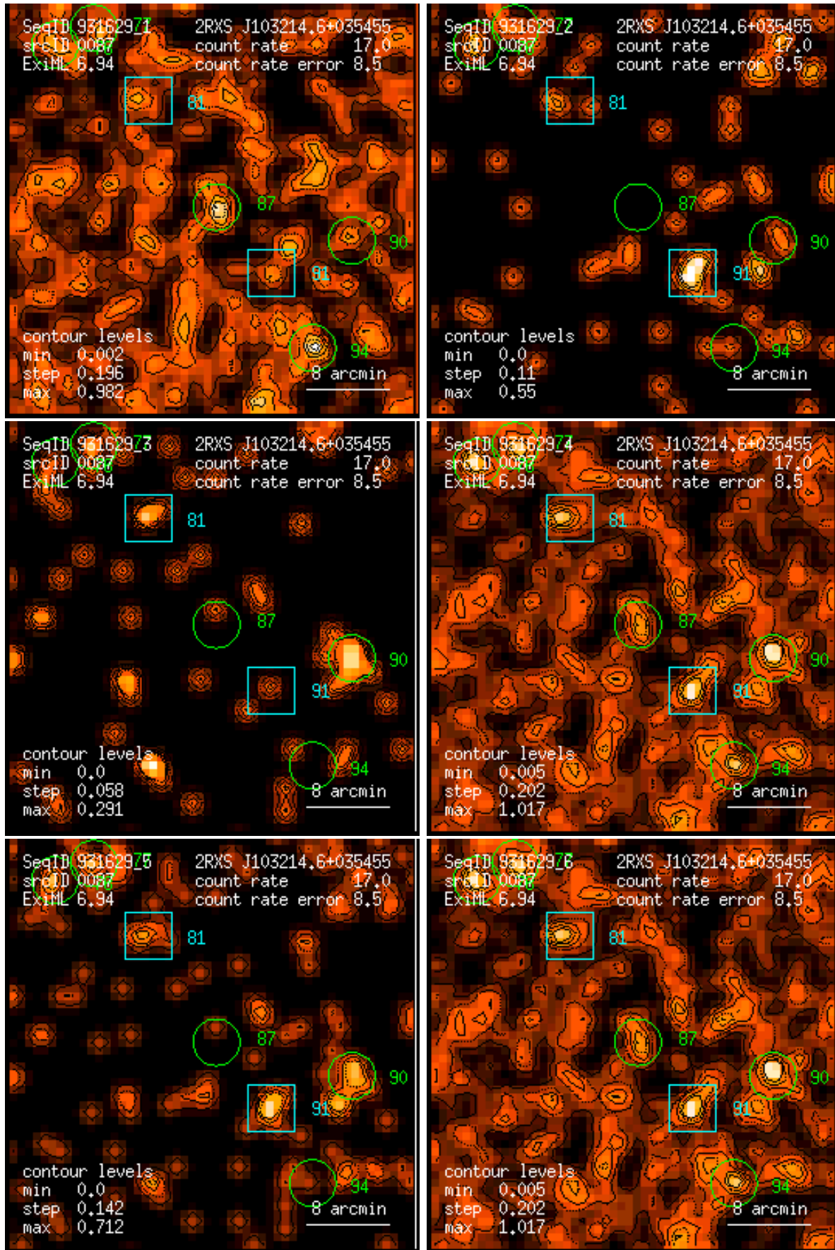
Figure 87: RASS 931629: detection 0087: band rate images, Gaussian filter: (1) PSPC channels 11 – 41, (2) 52 – 90, (3) 91 – 201, (4) 11 – 235, (5) 52 – 201, (6) 11 – 201. Broad band rates in counts/ks. Band rate contour levels in counts/ks/arcmin 2 .
