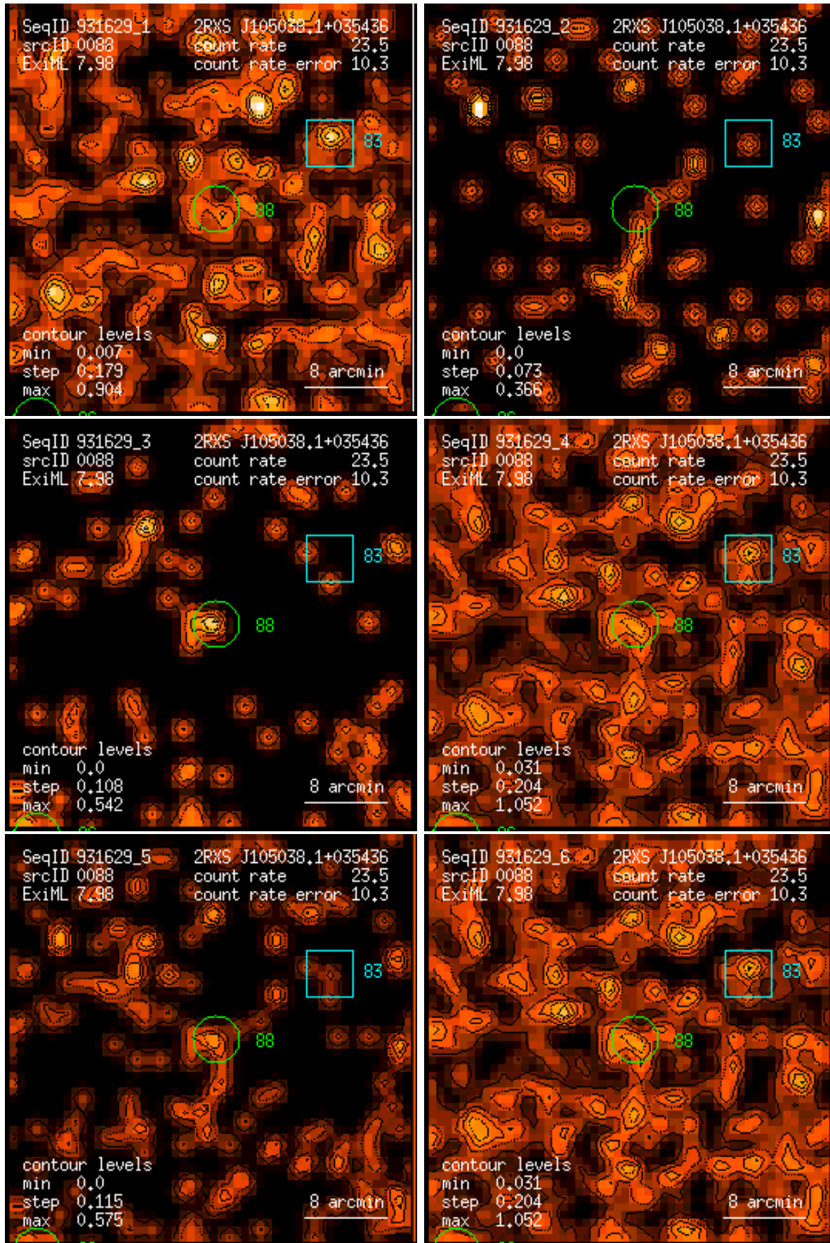
Figure 88: RASS 931629: detection 0088: band rate images, Gaussian filter: (1) PSPC channels 11 – 41, (2) 52 – 90, (3) 91 – 201, (4) 11 – 235, (5) 52 – 201, (6) 11 – 201. Broad band rates in counts/ks. Band rate contour levels in counts/ks/arcmin 2 .
