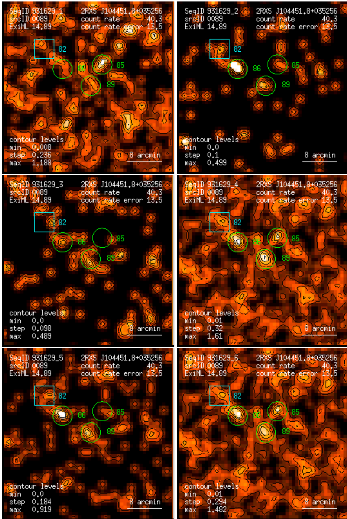
Figure 89: RASS 931629: detection 0089: band rate images, Gaussian filter: (1) PSPC channels 11 – 41, (2) 52 – 90, (3) 91 – 201, (4) 11 – 235, (5) 52 – 201, (6) 11 – 201. Broad band rates in counts/ks. Band rate contour levels in counts/ks/arcmin 2 .
