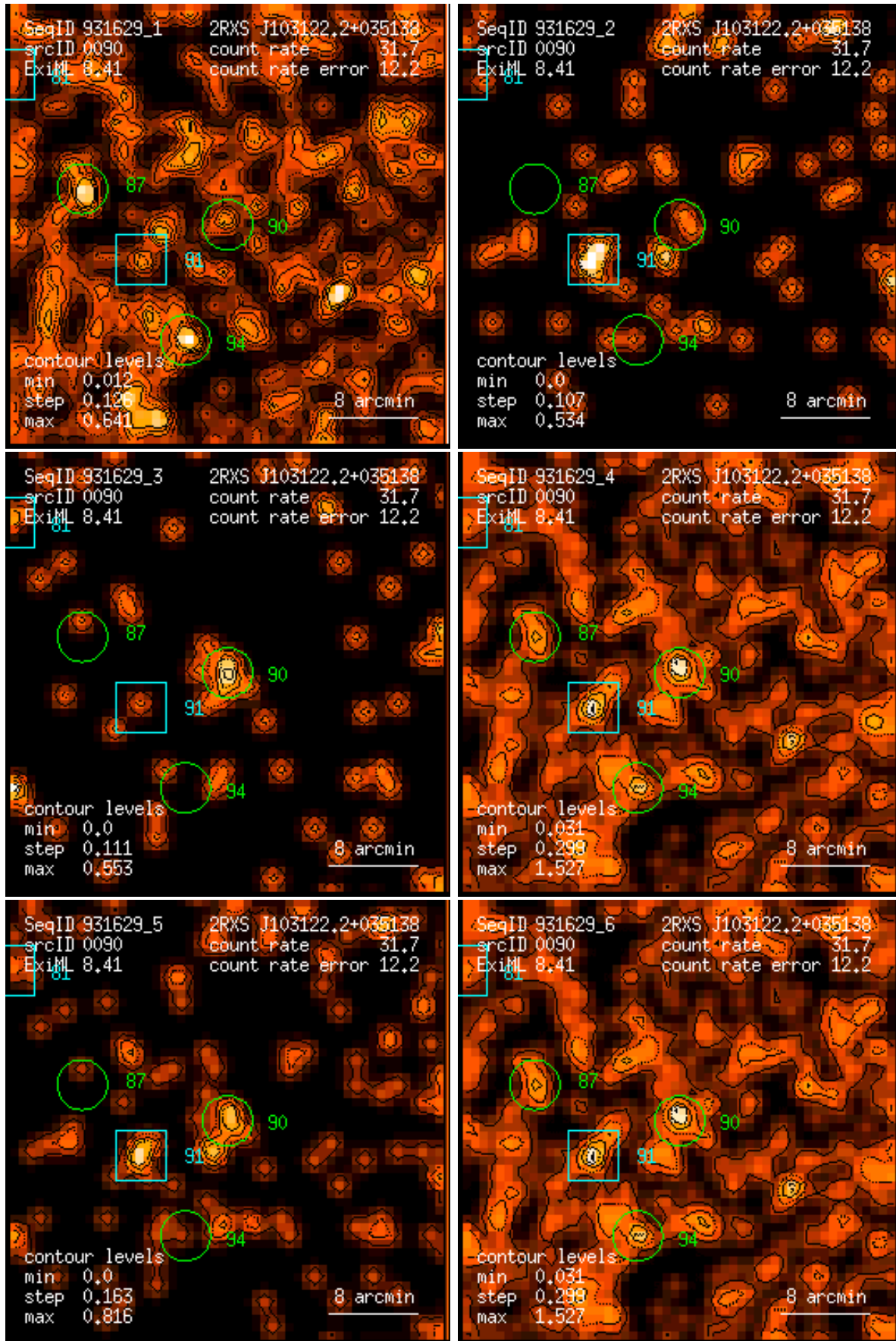
Figure 90: RASS 931629: detection 0090: band rate images, Gaussian filter: (1) PSPC channels 11 – 41, (2) 52 – 90, (3) 91 – 201, (4) 11 – 235, (5) 52 – 201, (6) 11 – 201. Broad band rates in counts/ks. Band rate contour levels in counts/ks/arcmin 2 .
