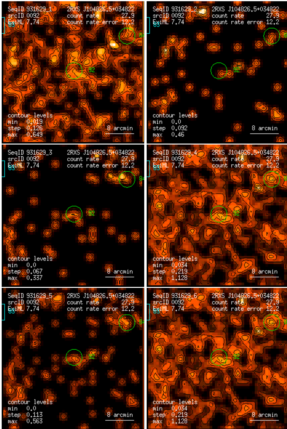
Figure 92: RASS 931629: detection 0092: band rate images, Gaussian filter: (1) PSPC channels 11 – 41, (2) 52 – 90, (3) 91 – 201, (4) 11 – 235, (5) 52 – 201, (6) 11 – 201. Broad band rates in counts/ks. Band rate contour levels in counts/ks/arcmin 2 .
