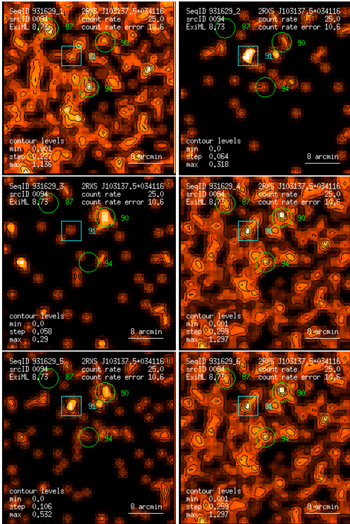
Figure 94: RASS 931629: detection 0094: band rate images, Gaussian filter: (1) PSPC channels 11 – 41, (2) 52 – 90, (3) 91 – 201, (4) 11 – 235, (5) 52 – 201, (6) 11 – 201. Broad band rates in counts/ks. Band rate contour levels in counts/ks/arcmin 2 .
