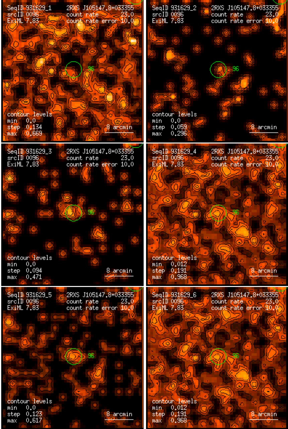
Figure 96: RASS 931629: detection 0096: band rate images, Gaussian filter: (1) PSPC channels 11 – 41, (2) 52 – 90, (3) 91 – 201, (4) 11 – 235, (5) 52 – 201, (6) 11 – 201. Broad band rates in counts/ks. Band rate contour levels in counts/ks/arcmin 2 .
