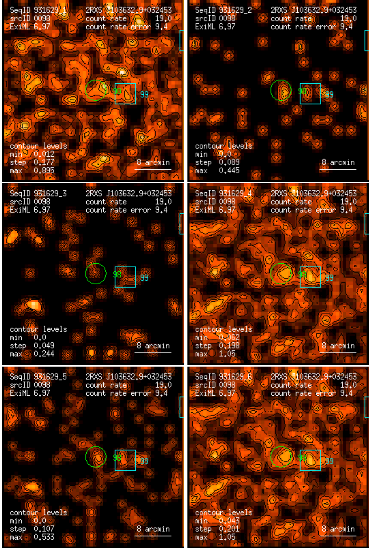
Figure 98: RASS 931629: detection 0098: band rate images, Gaussian filter: (1) PSPC channels 11 – 41, (2) 52 – 90, (3) 91 – 201, (4) 11 – 235, (5) 52 – 201, (6) 11 – 201. Broad band rates in counts/ks. Band rate contour levels in counts/ks/arcmin 2 .
