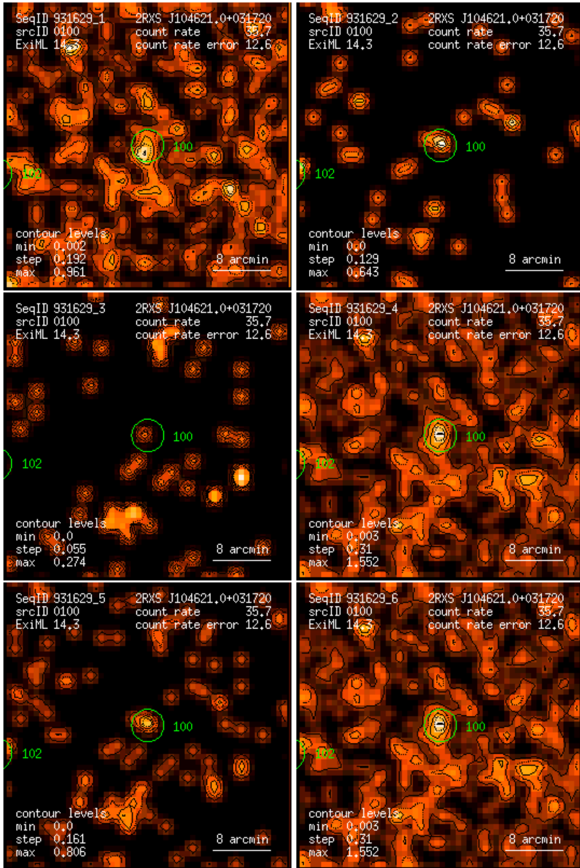
Figure 100: RASS 931629: detection 0100: band rate images, Gaussian filter: (1) PSPC channels 11 – 41, (2) 52 – 90, (3) 91 – 201, (4) 11 – 235, (5) 52 – 201, (6) 11 – 201. Broad band rates in counts/ks. Band rate contour levels in counts/ks/arcmin 2 .
