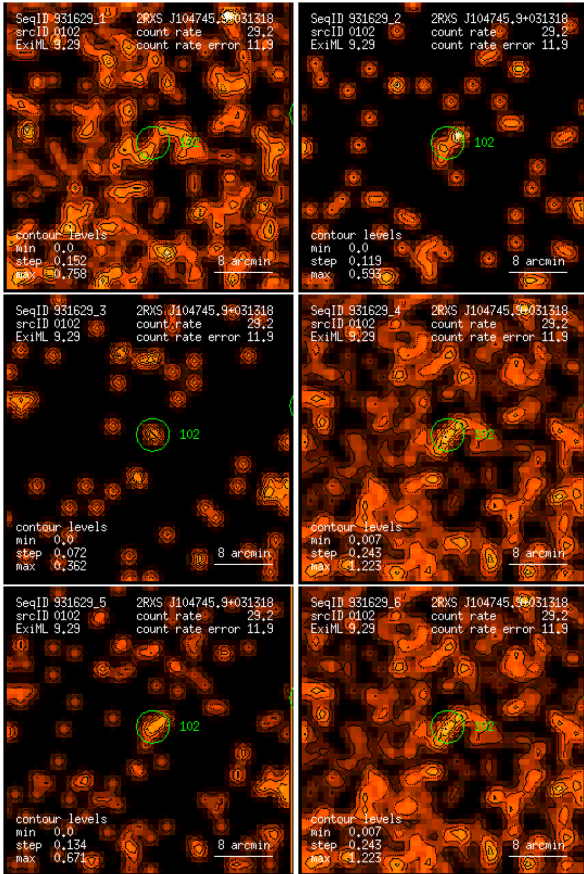
Figure 102: RASS 931629: detection 0102: band rate images, Gaussian filter: (1) PSPC channels 11 – 41, (2) 52 – 90, (3) 91 – 201, (4) 11 – 235, (5) 52 – 201, (6) 11 – 201. Broad band rates in counts/ks. Band rate contour levels in counts/ks/arcmin 2 .
