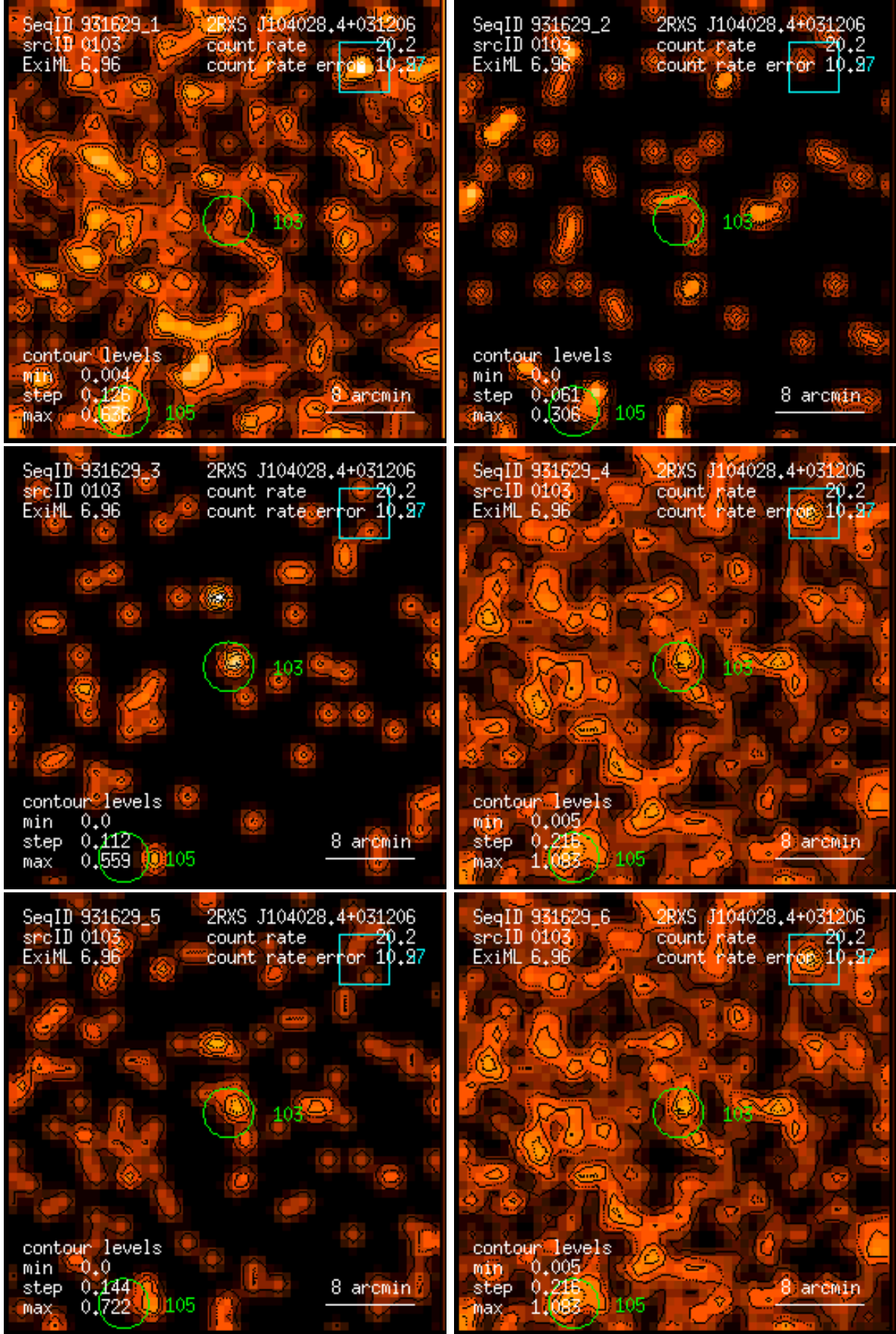
Figure 103: RASS 931629: detection 0103: band rate images, Gaussian filter: (1) PSPC channels 11 – 41, (2) 52 – 90, (3) 91 – 201, (4) 11 – 235, (5) 52 – 201, (6) 11 – 201. Broad band rates in counts/ks. Band rate contour levels in counts/ks/arcmin 2 .
