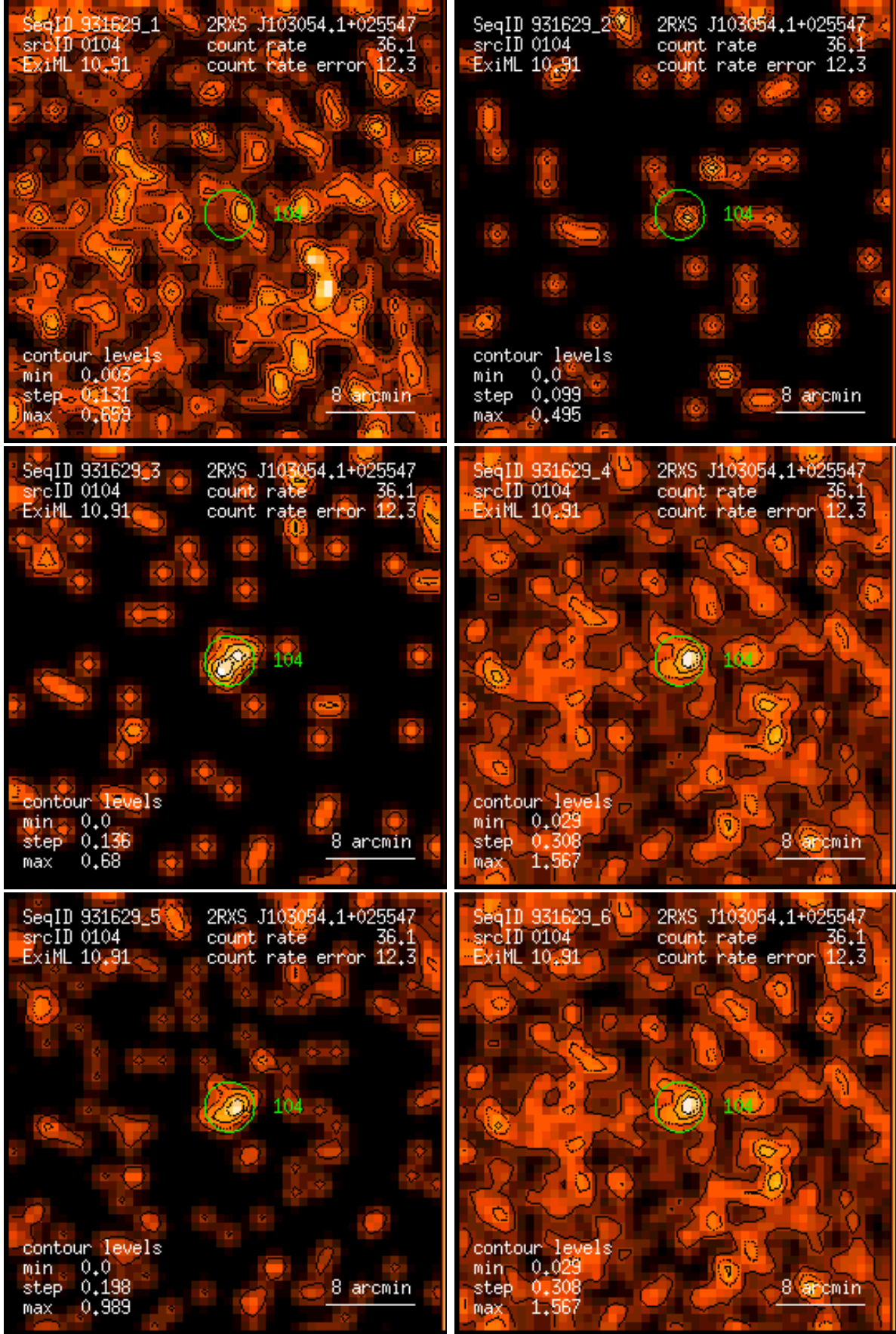
Figure 104: RASS 931629: detection 0104: band rate images, Gaussian filter: (1) PSPC channels 11 – 41, (2) 52 – 90, (3) 91 – 201, (4) 11 – 235, (5) 52 – 201, (6) 11 – 201. Broad band rates in counts/ks. Band rate contour levels in counts/ks/arcmin 2 .
