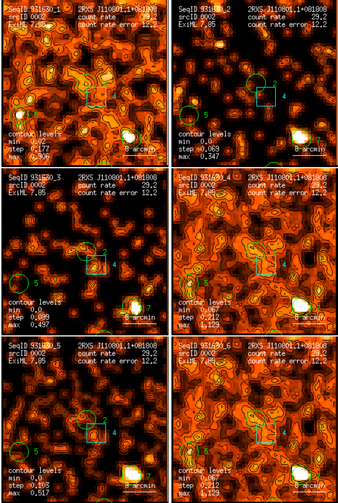
Figure 2: RASS 931630: detection 0002: band rate images, Gaussian filter: (1) PSPC channels 11 – 41, (2) 52 – 90, (3) 91 – 201, (4) 11 – 235, (5) 52 – 201, (6) 11 – 201. Broad band rates in counts/ks. Band rate contour levels in counts/ks/arcmin 2 .
