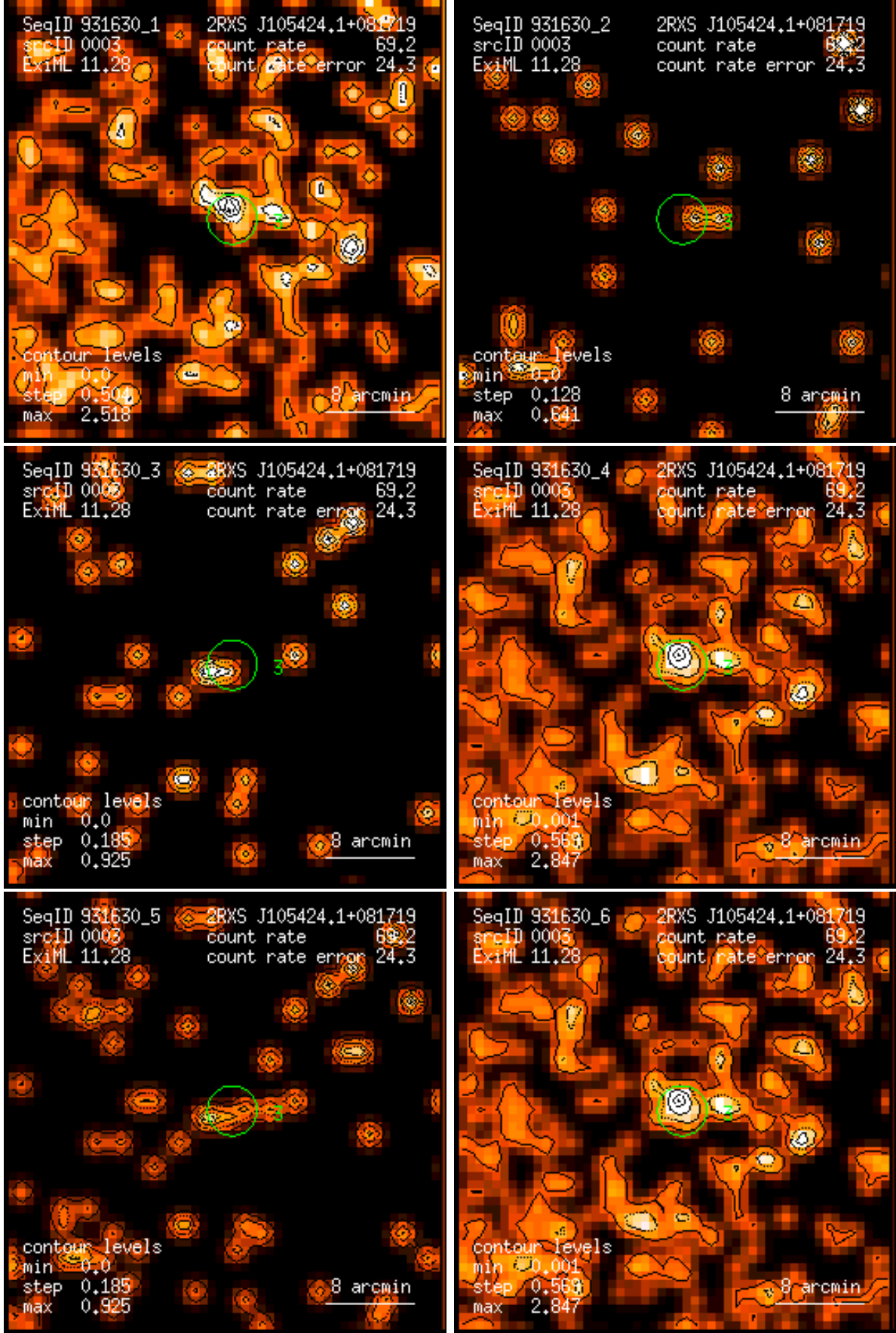
Figure 3: RASS 931630: detection 0003: band rate images, Gaussian filter: (1) PSPC channels 11 – 41, (2) 52 – 90, (3) 91 – 201, (4) 11 – 235, (5) 52 – 201, (6) 11 – 201. Broad band rates in counts/ks. Band rate contour levels in counts/ks/arcmin 2 .
