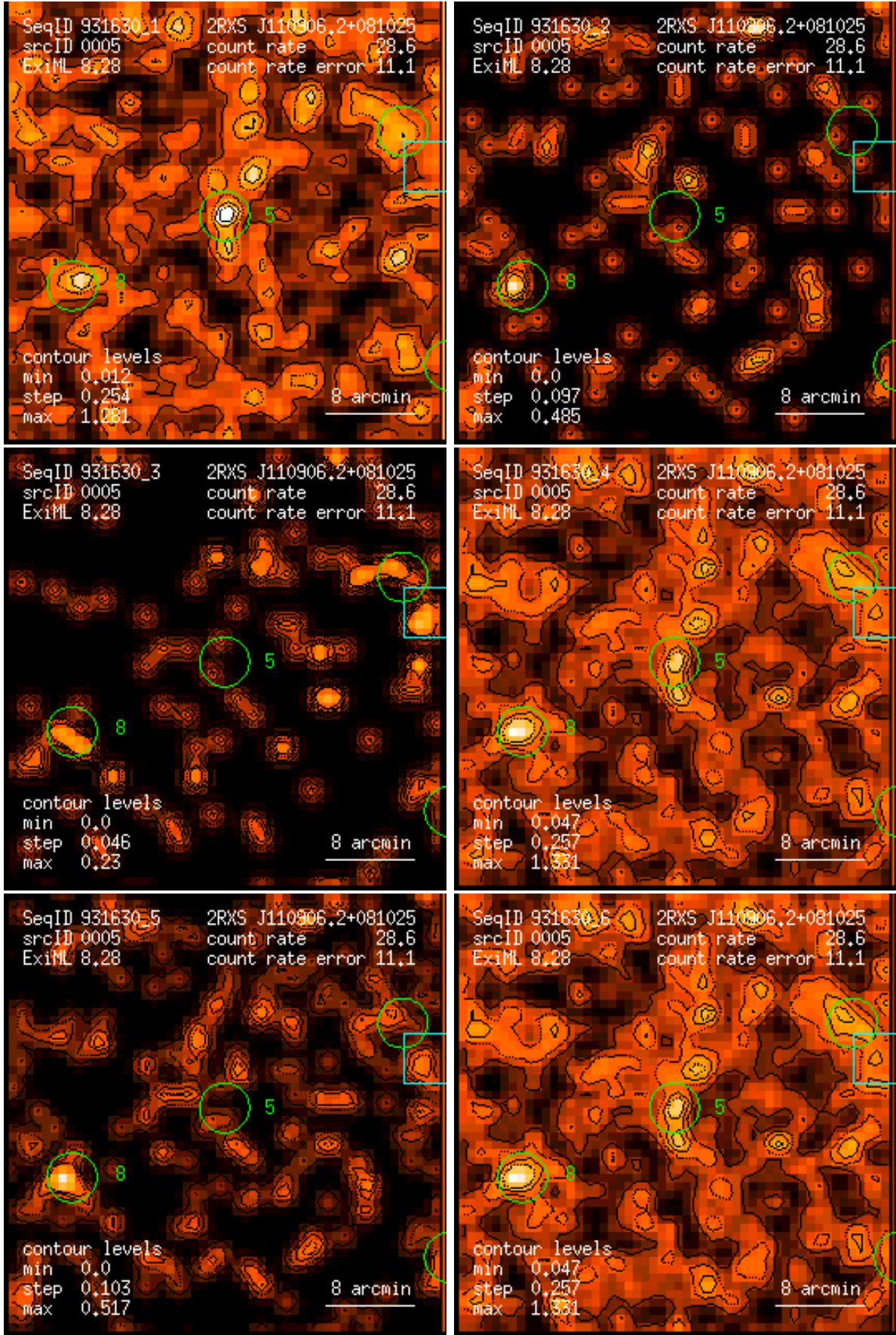
Figure 5: RASS 931630: detection 0005: band rate images, Gaussian filter: (1) PSPC channels 11 – 41, (2) 52 – 90, (3) 91 – 201, (4) 11 – 235, (5) 52 – 201, (6) 11 – 201. Broad band rates in counts/ks. Band rate contour levels in counts/ks/arcmin 2 .
