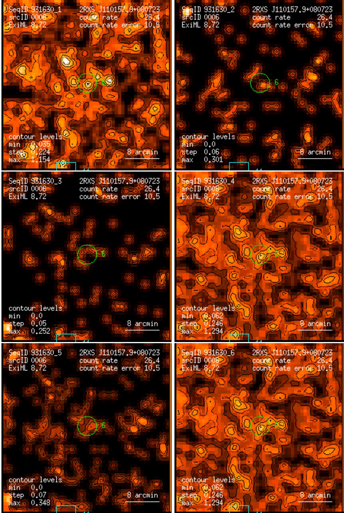
Figure 6: RASS 931630: detection 0006: band rate images, Gaussian filter: (1) PSPC channels 11 – 41, (2) 52 – 90, (3) 91 – 201, (4) 11 – 235, (5) 52 – 201, (6) 11 – 201. Broad band rates in counts/ks. Band rate contour levels in counts/ks/arcmin 2 .
