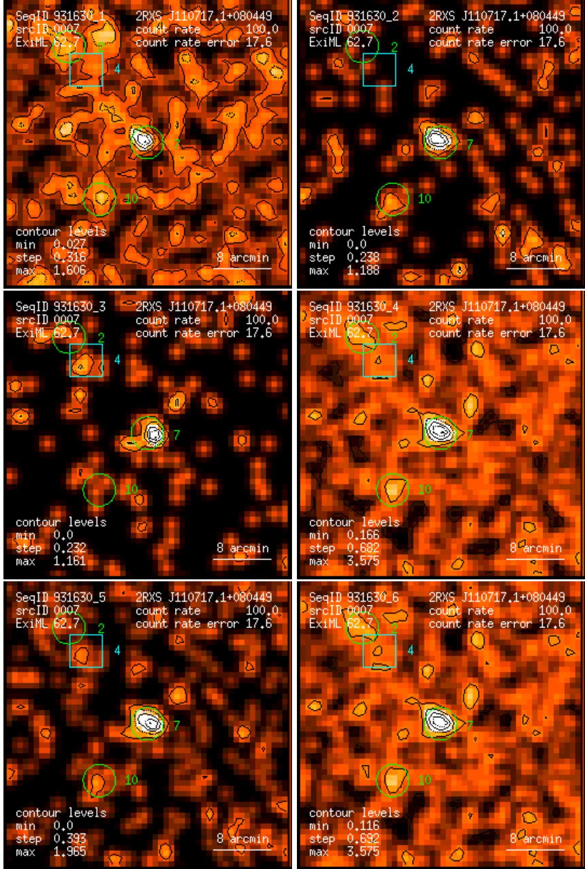
Figure 7: RASS 931630: detection 0007: band rate images, Gaussian filter: (1) PSPC channels 11 – 41, (2) 52 – 90, (3) 91 – 201, (4) 11 – 235, (5) 52 – 201, (6) 11 – 201. Broad band rates in counts/ks. Band rate contour levels in counts/ks/arcmin 2 .
