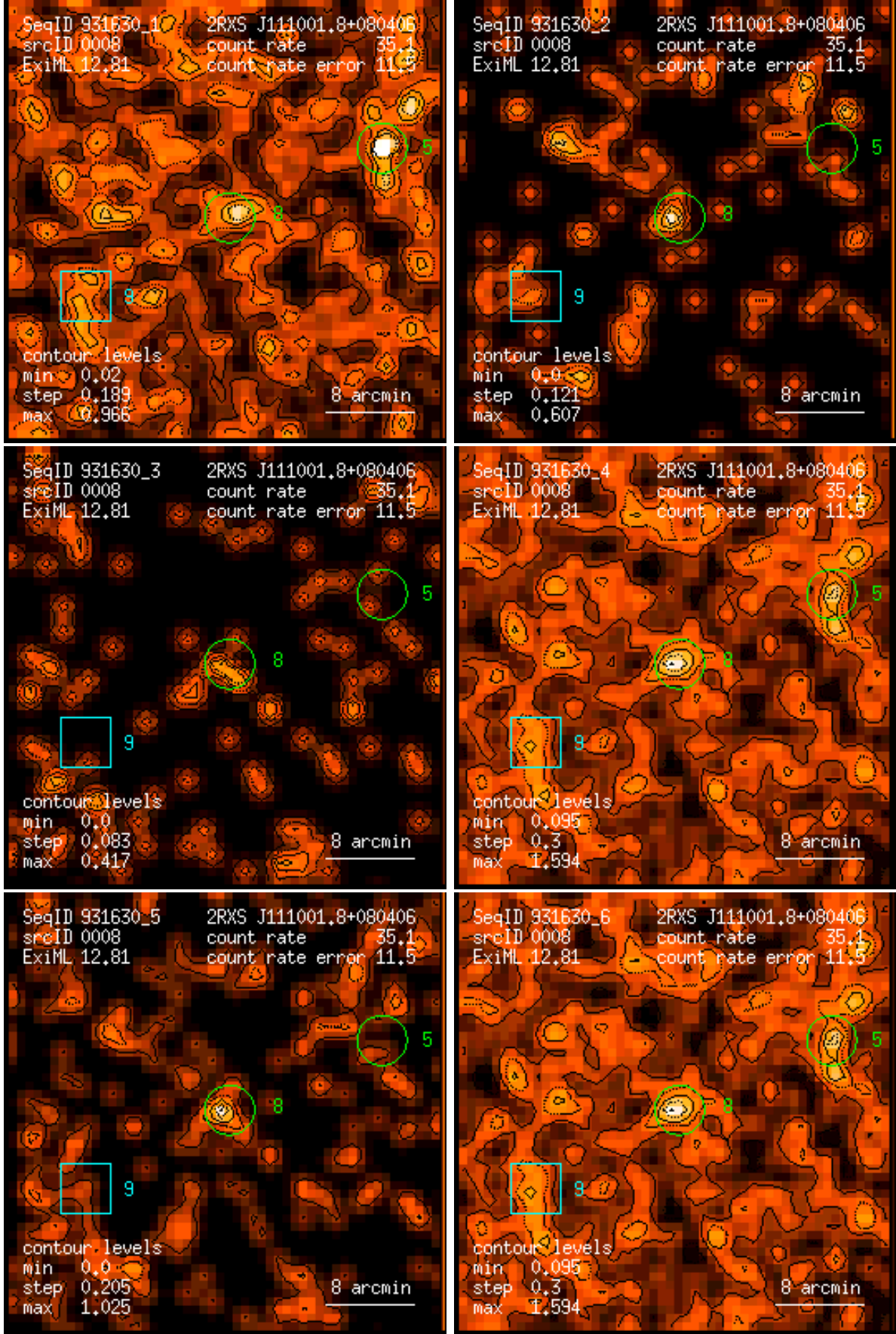
Figure 8: RASS 931630: detection 0008: band rate images, Gaussian filter: (1) PSPC channels 11 – 41, (2) 52 – 90, (3) 91 – 201, (4) 11 – 235, (5) 52 – 201, (6) 11 – 201. Broad band rates in counts/ks. Band rate contour levels in counts/ks/arcmin 2 .
